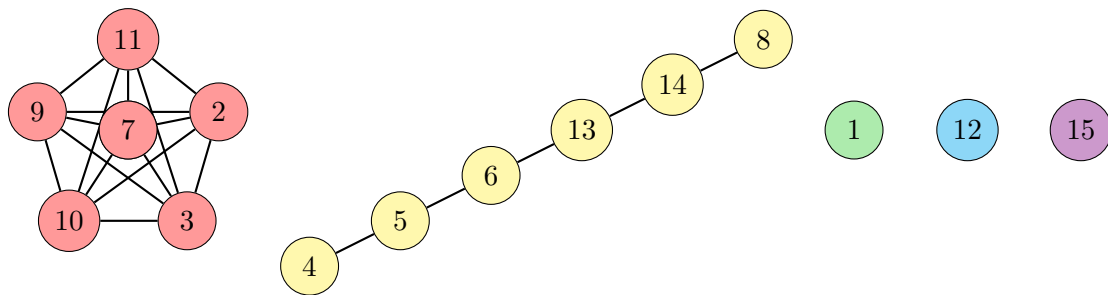
Figure 8.2.3: The filtered complex for Wiegenslied Op. 49-4 at a scale of 13%. There are two main connected components made of the two types of musical bars in the score (a half note with two quaver ones and two quarter notes with two quaver ones), and three made of one vertex, bar \mathcal{B}_1 (the beginning), bar \mathcal{B}_{15} (the ending) and bar \mathcal{B}_{12} (a transition made of three quarter notes).
