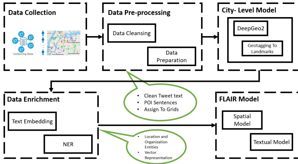
Figure 5.7: Implementation Pipeline
