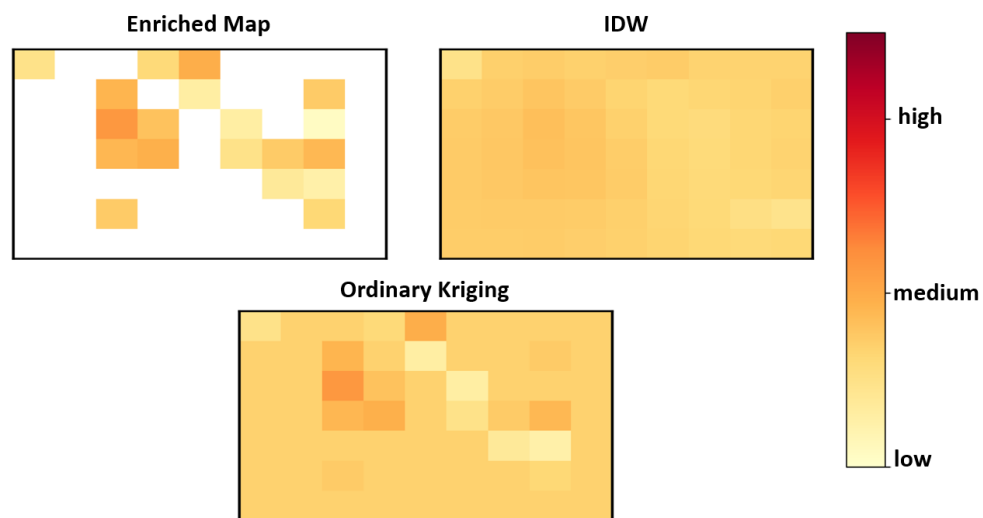
Figure 4.16: IDW and Ordinary Kriging 500m x 500m - Versailles (Cluster 2)
