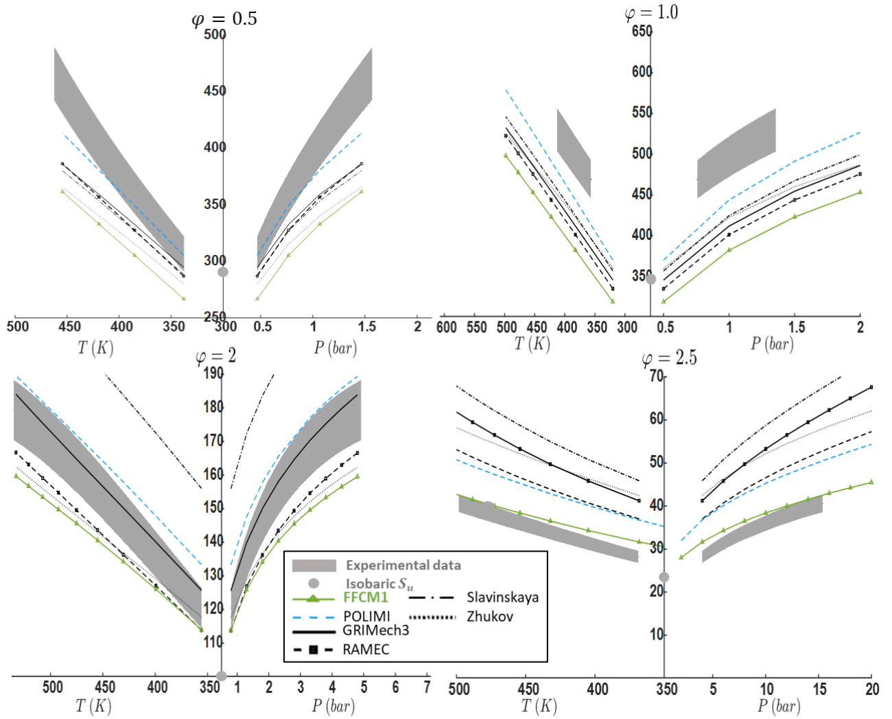
Figure 113: Flame speed S_u [cm.s -1 ] for CH_4 / O_2 mixtures at various equivalence ratios \phi (thickened traces) as a function of T and P compared to several kinetic mechanisms (lines). Single symbols are for experimental isobaric flame speeds.
