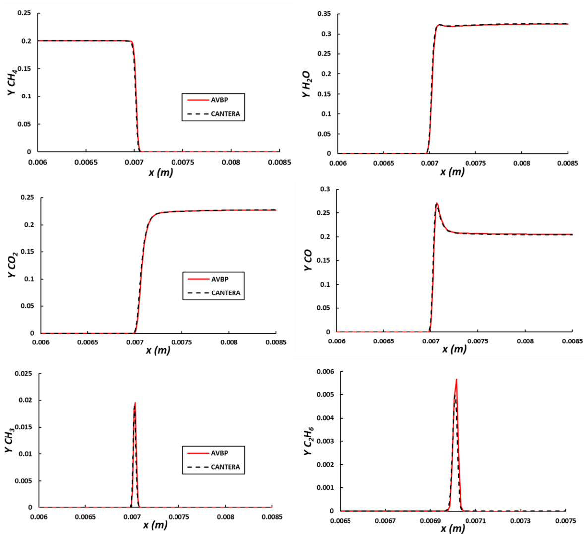
Figure 76: Profiles of mass fractions of various species for a 1D premixed \text{CH}_4 / \text{O}_2 flame at \phi=1 and P=1.36 bar (target 2 of Table 15) computed with CANTERA vs pseudo 1D AVBP calculations with the Polimi Opti ARC mechanism – zoomed on the flame region
