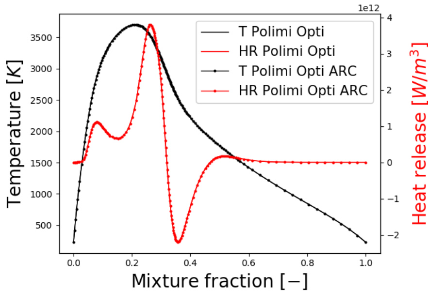
Figure 68: Profile of a 1D highly strained ( \chi = 1500 \text{ s}^{-1} ) diffusion flame at high pressure ( P = 120 \text{ bar} ) showing heat release rate and temperature evolution as a function of the mixture fraction. Comparison between Polimi Opti and the ARC reduced schemes for the REST HF-10 test case
