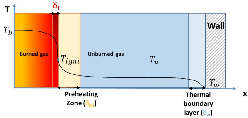
Figure 26 : Illustration of a premixed laminar flame structure
