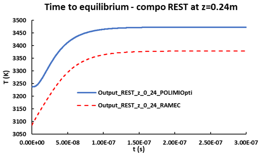
Figure 111: CANTERA OD computation with burnt gas composition at z=0.24m for both chemistries
