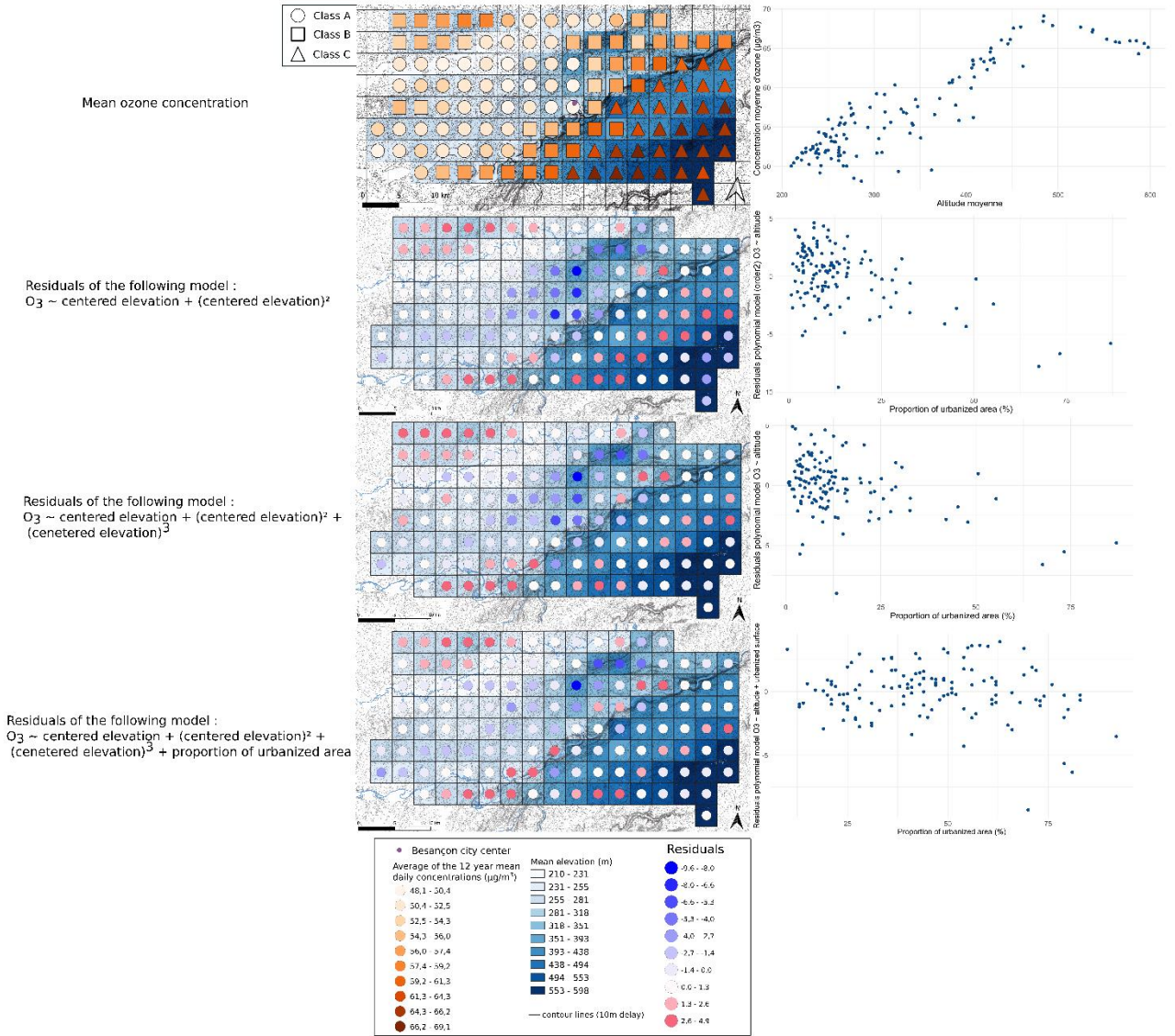
Figure A.7: Decomposition of the modelled relationship between ozone concentration and elevation, and spatialization of the residuals of the regressions.
