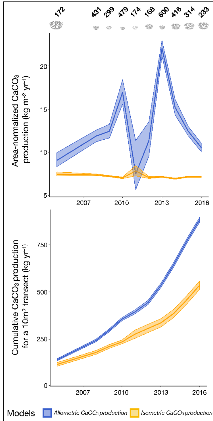
Figure 3.4 | Coral community \text{CaCO}_3 production estimates of a 10\text{m}^2 portion of reef substrate in Mo'orea from 2005 to 2016 according to the isometric versus allometric coral \text{CaCO}_3 production models. A. \text{CaCO}_3 production rate ( \text{kg m}^{-2} \text{yr}^{-1} ), B. cumulative \text{CaCO}_3 production ( \text{kg yr}^{-1} ). Estimates are bounded by a 95% confidence interval. Coral symbols on top indicate changes in average coral colony size, and numbers indicate coral colony density per 10\text{m}^2 of reef surface area.
