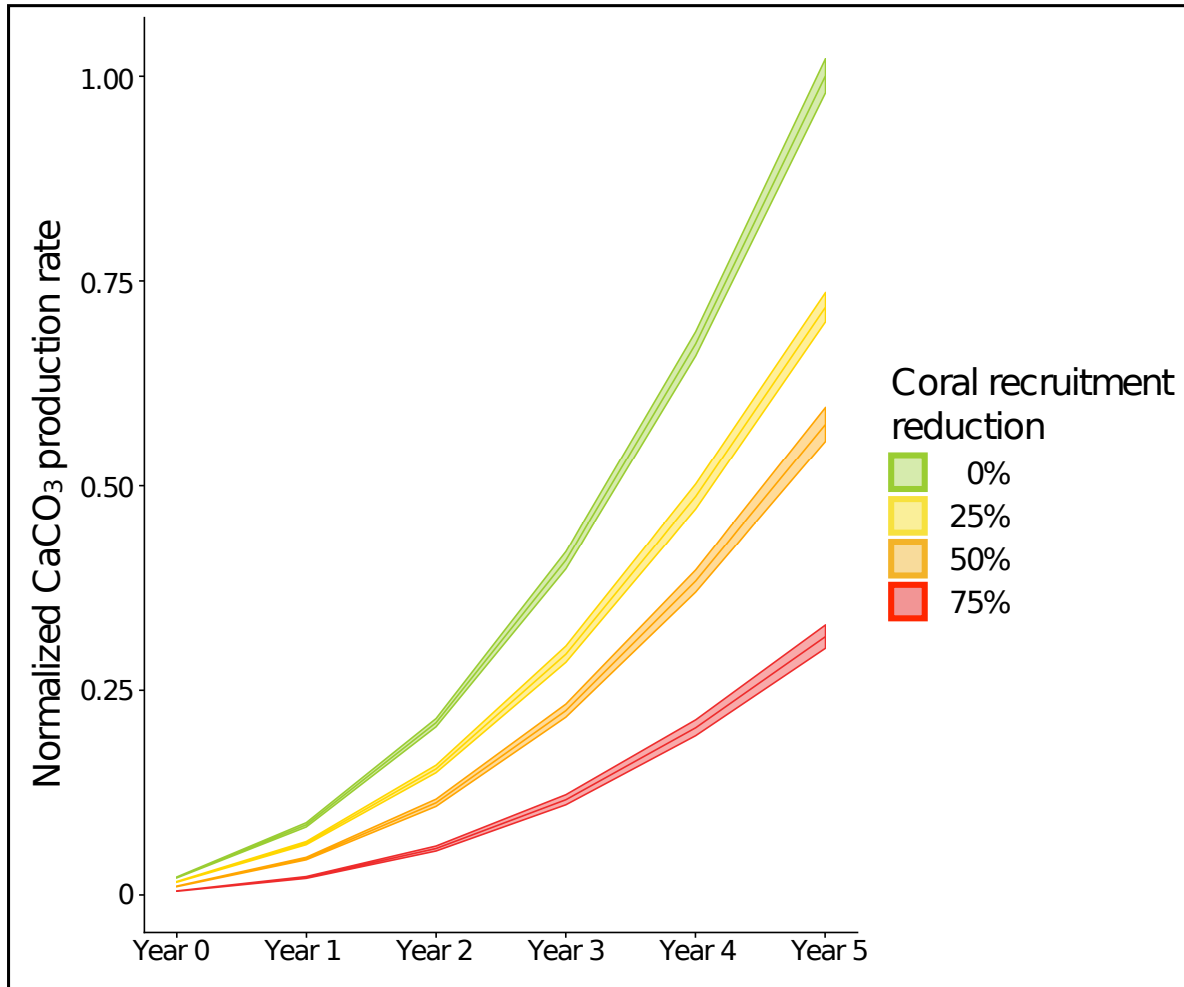
Figure 3.5 | Normalized \text{CaCO}_3 production trajectories according to four scenarios of coral recruitment over five years during reef recovery. A multi-species, open-population integral projection model was used to predict the recovery dynamics of an assemblage of three coral genera ( Acropora , Pocillopora and Porites ) based on coral demographic performance (in recruitment, growth, and survival) measured in Mo'orea. The four scenarios predicted different rates of coral recruitment reduction as compared to current levels (0%, 25%, 50% and 75% reductions). \text{CaCO}_3 production rates were estimated from model predictions of coral abundance, composition and size distribution (Figure S5, combined with the allometric \text{CaCO}_3 production functions estimated in Mo'orea (Fig. 1). \text{CaCO}_3 production rates were normalized relative to the highest value (scenario 0% reduction at year 5; green curve).
