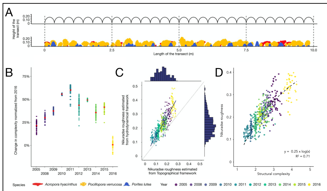
Figure S5.5 | Definition of the Nikuradse estimates ( k_n ) A. Definition of the average coral height within a 10\text{m}^2 transect and illustration of the k_n estimates equivalent above. Acropora hyacinthus were represented in red, Pocillopora cf. verrucosa in orange and Porites lutea in blue B. Change in complexity from 2005 to 2016. The standard year has been selected for 2016 because the highest structural complexity estimates were defined this year. Red points represent the average for each year. C. Scatterplot between k_n estimates defined by the ‘topographical approach’ and k_n estimates defined by the ‘hydrodynamical approach’. D. Relationship between structural complexity and K_n estimates. The relationship is written as k_n = 0.25 \times \log(\text{Structural complexity}) .
