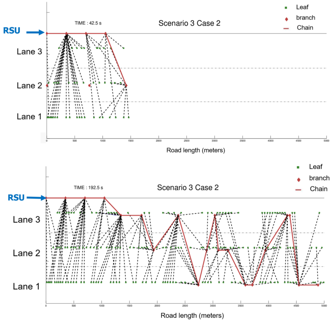
Figure 2.15: S3- UC2- Chain formation for simulation B when leaving a RSU area at different times (42,5 sec) and (192,5 sec)
