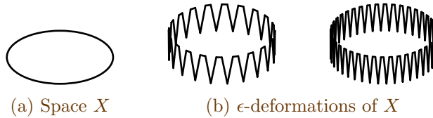
Figure 5.4: Illustration of the proof of Theorem 5.6.2
