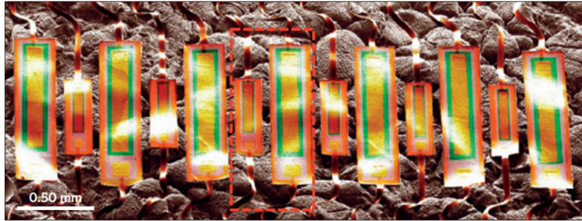
Figure 1.16: Thin, compliant modulus sensor (CMS) based on nanoribbons of PZT in arrays of mechanical actuators and sensors [35].
