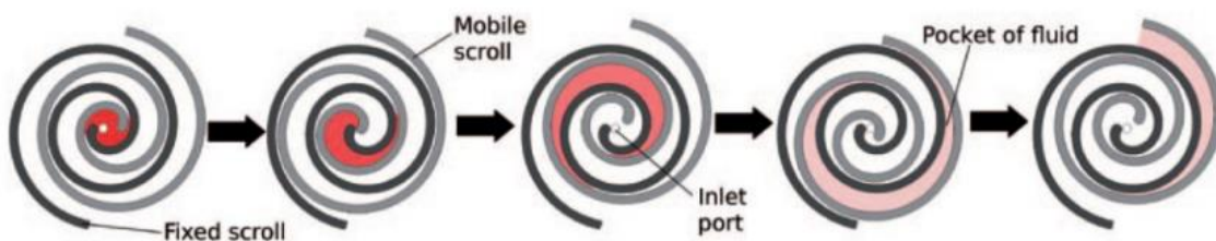
Fig. 2.14 - Scroll expander working principle [83].
