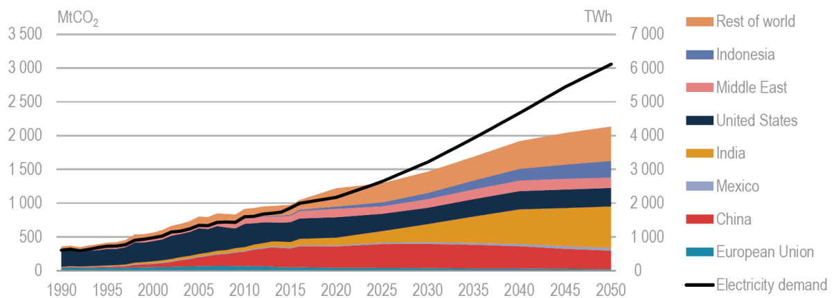
Fig. 1.3 - Electricity demand for space cooling and resulting CO 2 emissions in the 2016 IEA Baseline Scenario [21].
