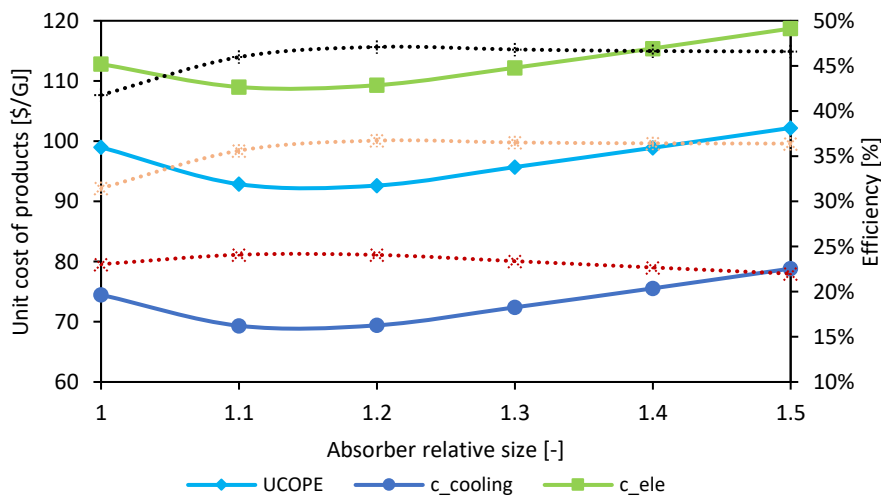
Fig. 5.10 - Impact of the absorber area with respect to the scaled up plant in the base case operating point for c_{fuel} = 15\text{ \$/GJ} .
