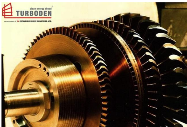
Fig. 2.9 - Example of ORC axial turbine [71] and velocities triangle [69].
