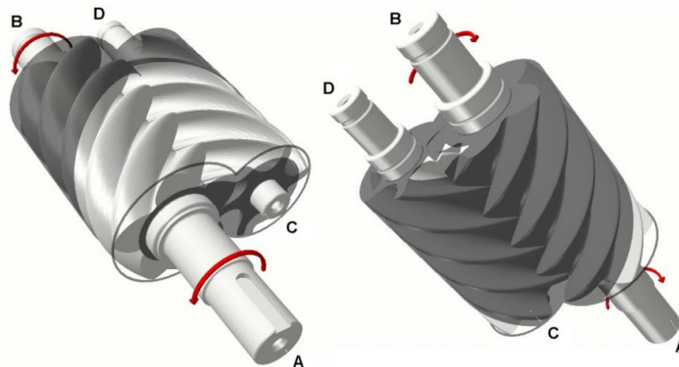
Fig. 2.11 - Screw expander [74].
