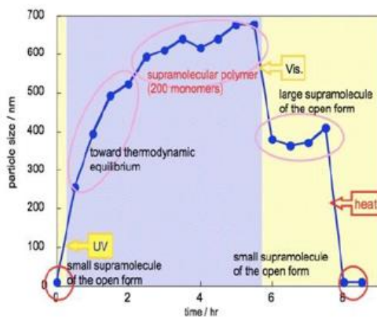
Figure 20. DLS particle size change of the photoswitch aggregation upon irradiation with UV and visible light [45].
