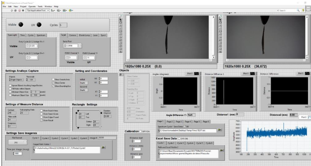
Figure 38. Display of the displacement measurement program developed for image storage, processing, and analysis, as well as manipulation of power and irradiation time of the films.
