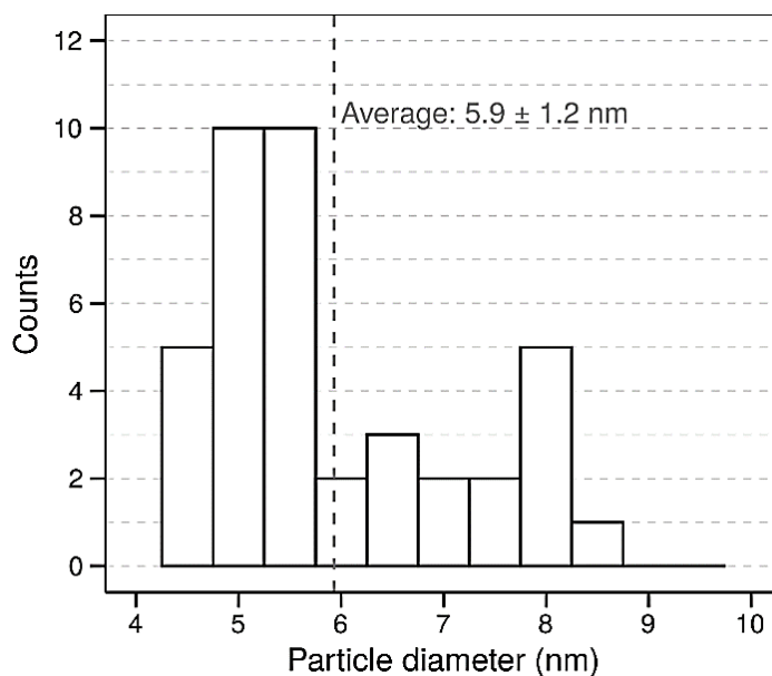
Figure 4.39. Size distribution histogram of the smallest particles present in HTNi2.5_5.
