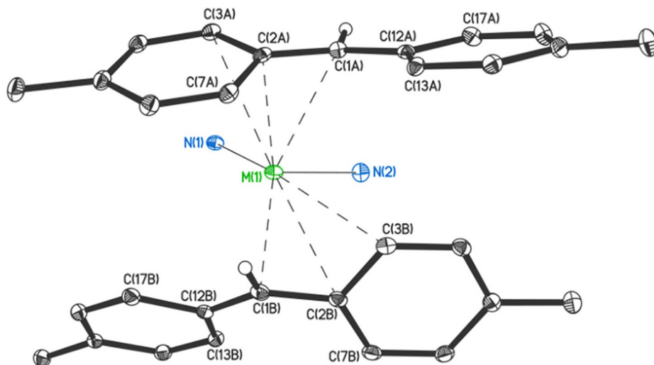
Fig. 9 Molecular structure of a representative complex [(p\text{-}^i\text{Bu-C}_6\text{H}_4)_2\text{CH}]_2\text{Ln}(\text{L})_n ( 14' Ln , M = Ln = Sm, Yb). Ellipsoids are set at the 30% probability, hydrogen atoms, methyl groups of i -Bu-substituents, and carbon atoms of TMEDA molecules are omitted for clarity. Reprinted from Selikhov, A. N.; Plankin, G. S.; Cherkasov, A. V.; Shavyrin, A. S.; Louyriac, E.; Maron, L.; Trifonov, A. A. Inorg. Chem. 2019 , 58 , 5325–5334, with the authorization of the American Chemical Society.
