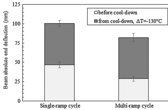
Figure 2.59 The deformation of specimen from Oleksandr et al. [85]
