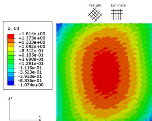
Figure 4.29 The simulation of cross-ply laminate with a peel-ply oriented at 45 °.
