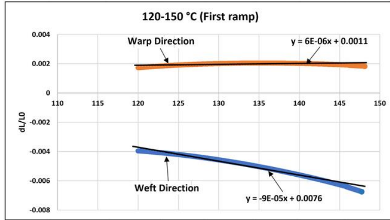
Figure 4.16 Changes in the strains of cured resin impregnated peel-ply as a function of temperature between 120-150 °C.
