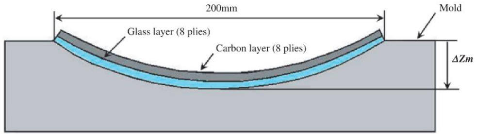
Figure 4.42 Compensated mould for hybrid composite beam. [65]
