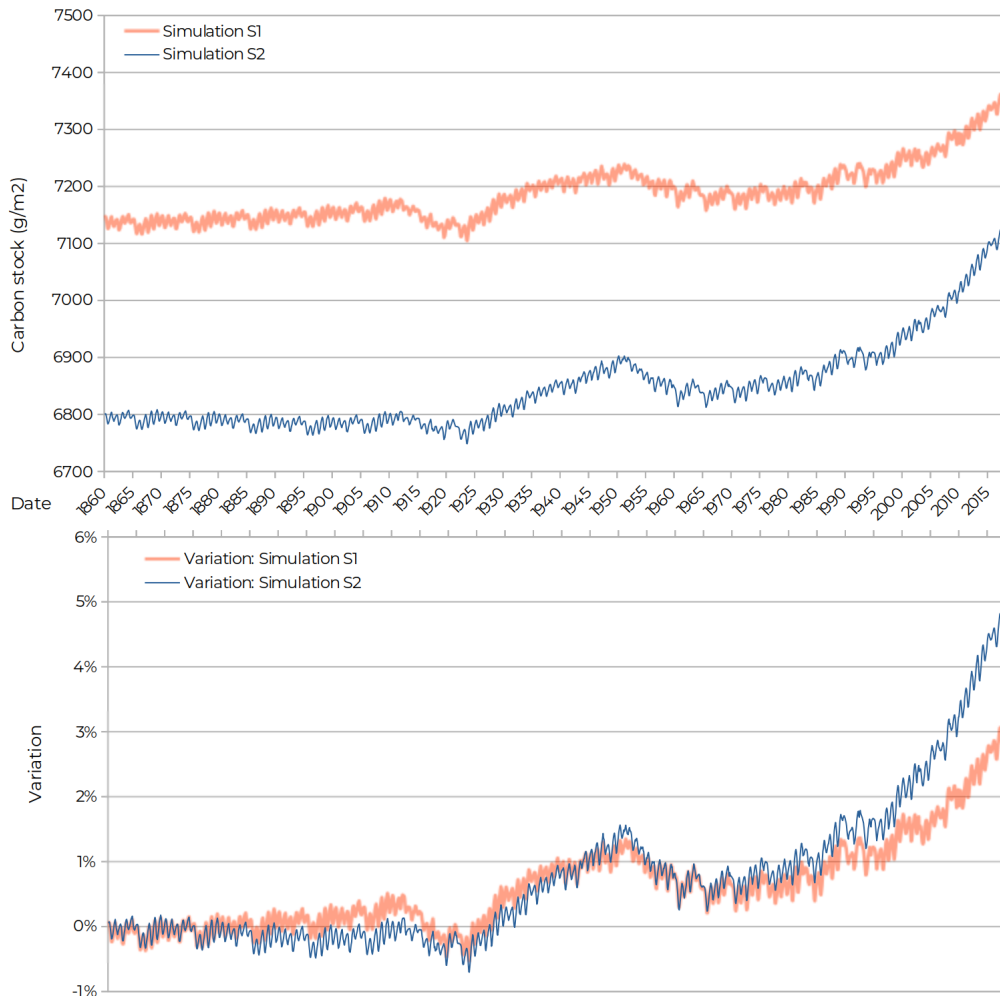
Figure 2.10: Results for the depositional site: absolute values of carbon stock (g/m 2 ) (top), relative difference compared to the stock at the first simulation month (bottom). Scenario S1 contains all ETD fluxes, while scenario S2 represents the dynamics of the original LSM.
