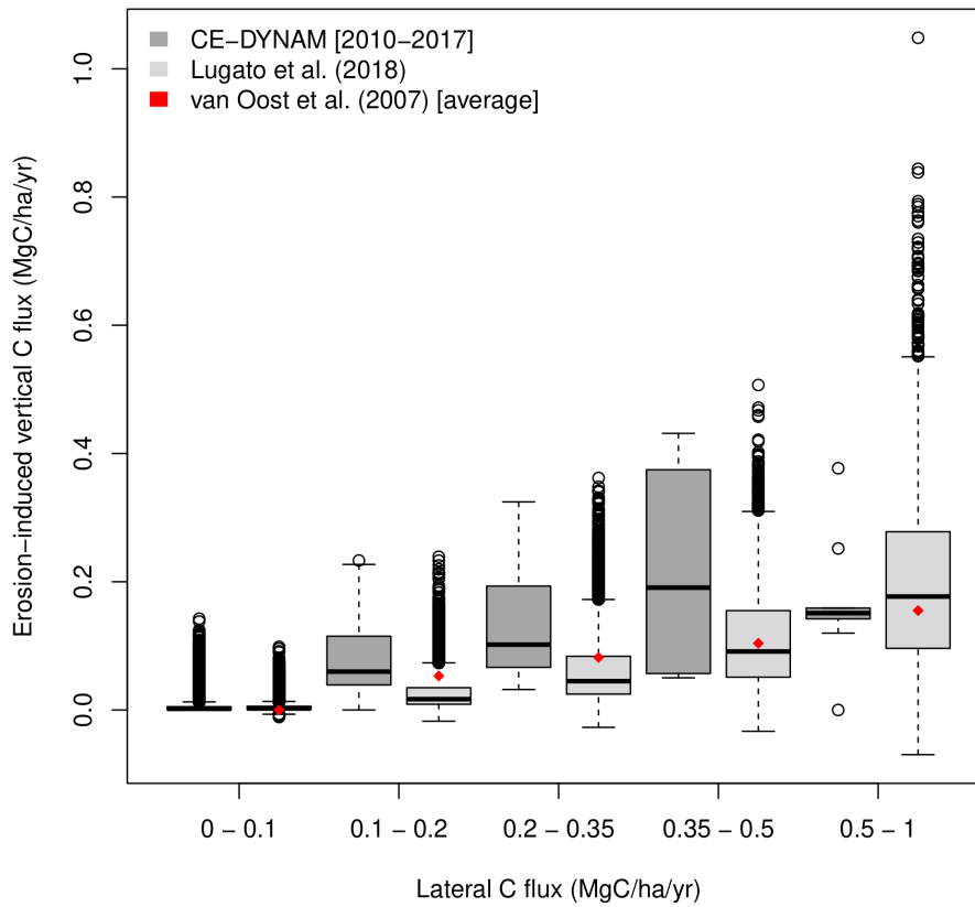
AP B.3: Comparison between the dynamic replacement for croplands in CE-DYNAM and other works (Lugato et al., 2018; Oost et al., 2007)
