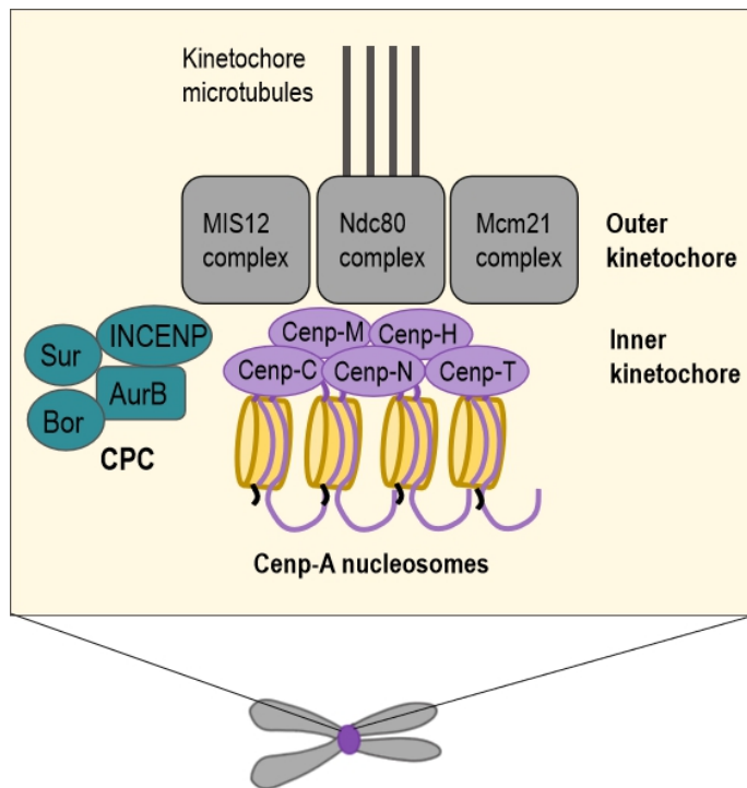
Figure 18. The kinetochore.
