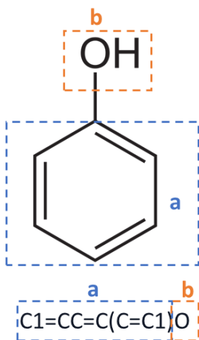
Figure 20: Structure of phenol and its respective Canonical SMILES.
