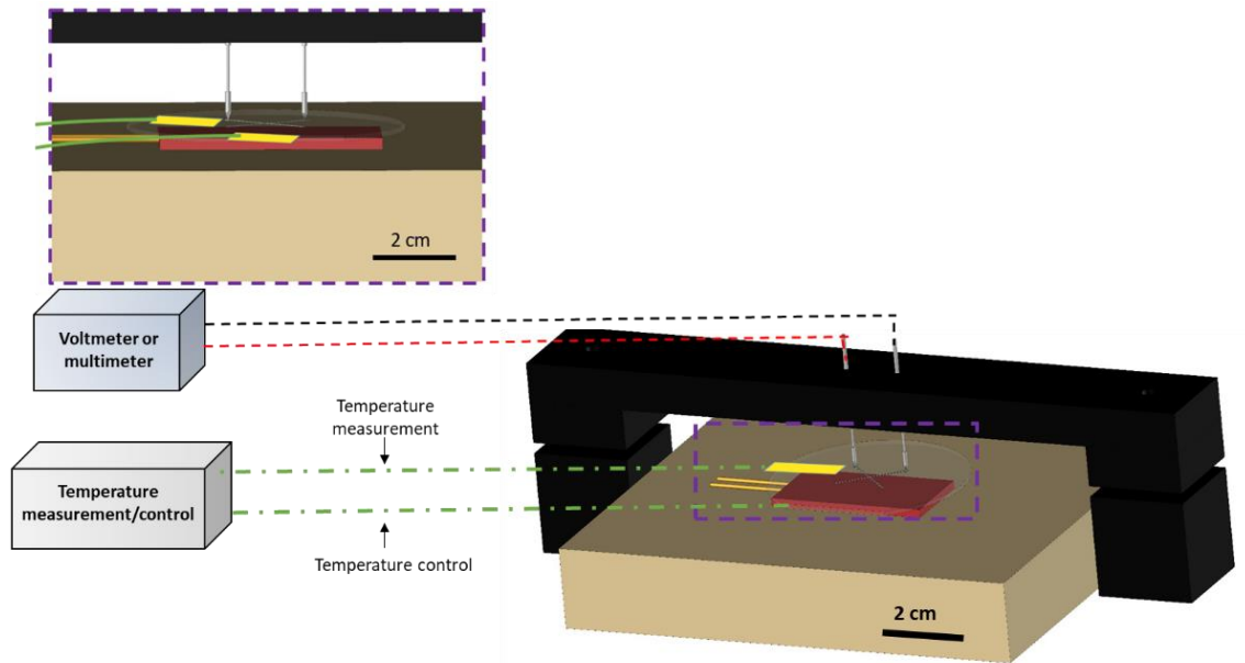
Figure 47: Illustration of the resistance and voltage set-up.
