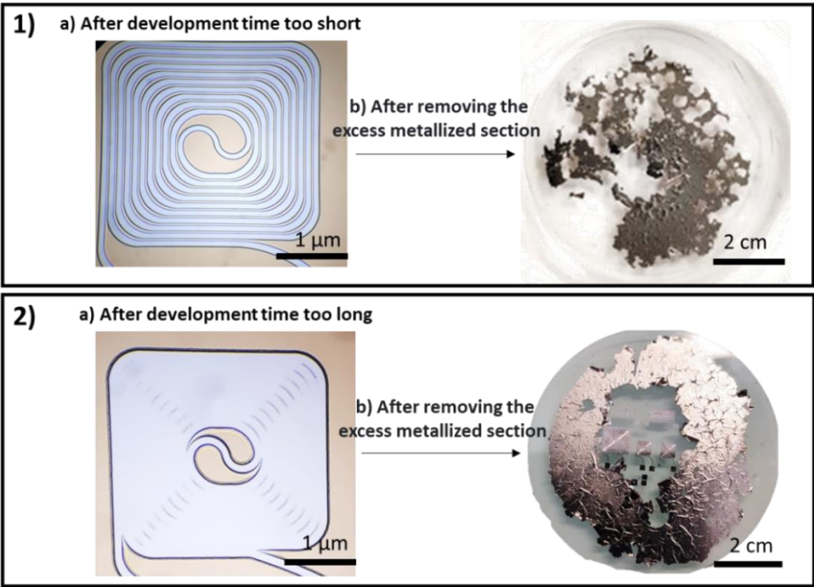
Figure 43: Two examples of 1) a) too short development time (< 20 seconds) with well design patterns followed by b) removal of the exceeding metallized section causing the pattern to spread out completely. 2) a) too long development time (> 60 seconds) loss of resolution followed by b) removal of the exceeding metallized section without the spread out of the pattern.
