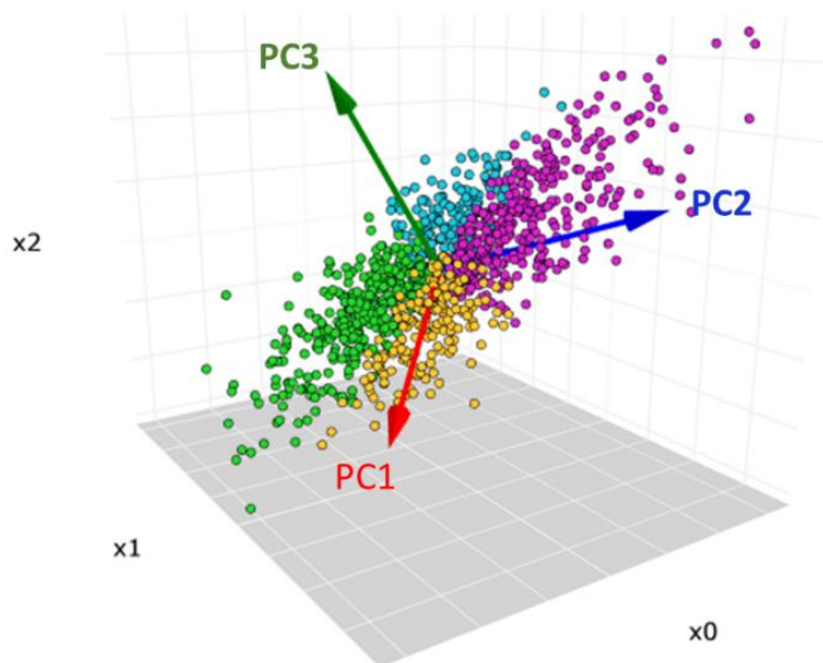
Figure 93: A 3-dimensional data set space. The red, blue, green arrows are the direction of the first, second, and third principal components, respectively. Extracted from ref [274].
