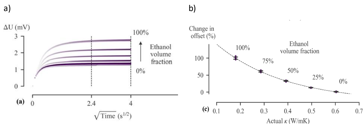
Figure 18: a) Thermal pulses applied while different water/ethanol mixtures were present in the microchannel. Linear curve fits were performed on the marked time interval. The raw data indicates that the various water/ethanol mixtures have an impact on the offset in the transient curves. b) Offset values are plotted as a function of the \lambda_L of the water/ethanol mixtures as found in literature. An exponential relation is observed (reproduced from ref. [42]).
