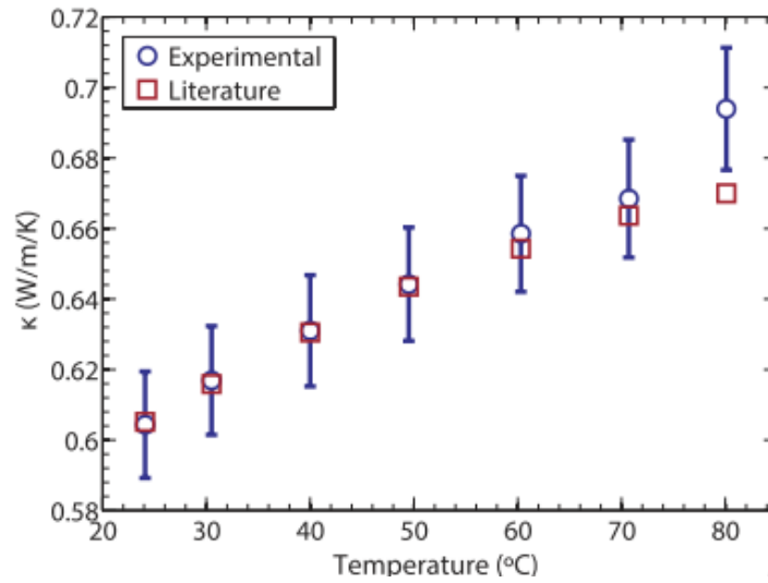
Figure 14: Temperature-dependent thermal conductivity DI water, with comparison to literature values (reproduced from ref. [134]).
