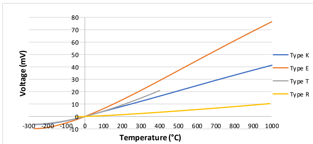
Figure 10: Voltage variation in function of temperature for different thermocouples.
