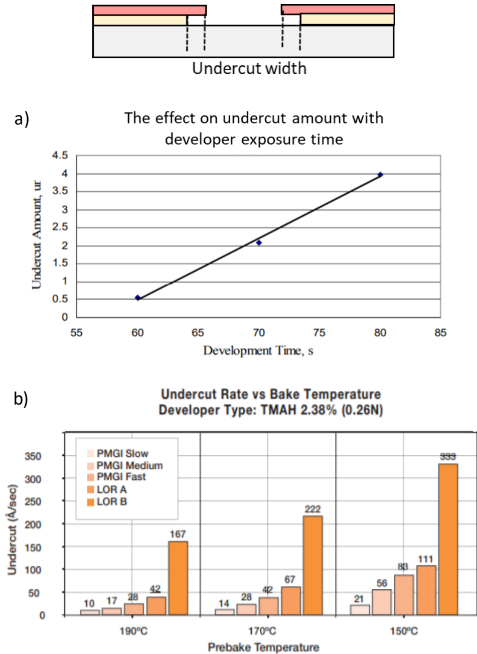
Figure 41: Effect on undercut while modifying develop time and bake temperature [233].
