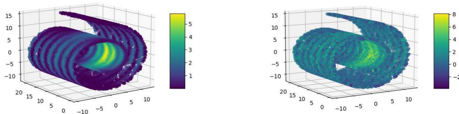
(a) Original function
