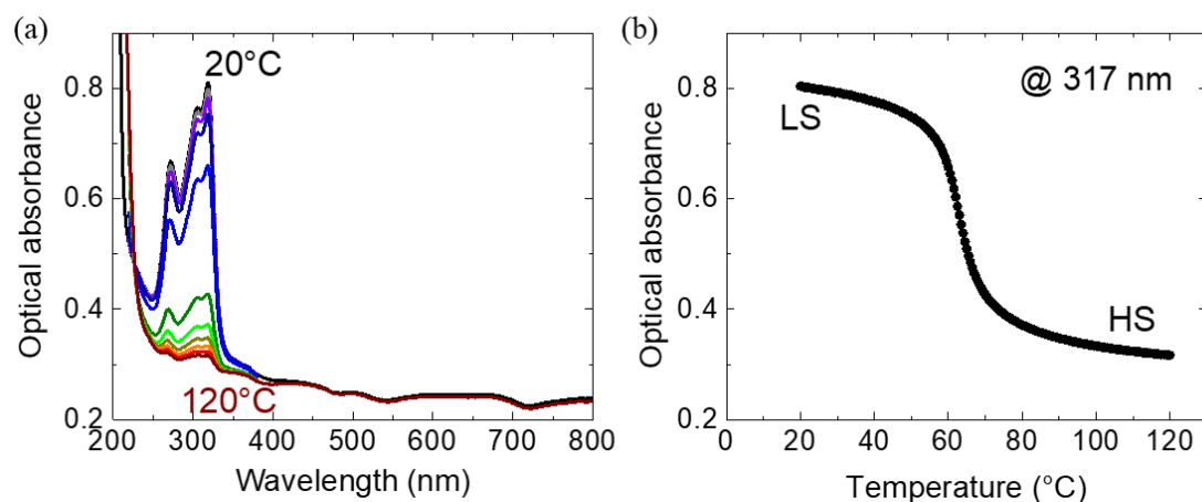
Figure 2.9. (a) Optical absorbance spectra of a 138-nm-thick film of the complex 1 , acquired at selected temperatures between 20 and 120 °C. The films were deposited on fused-silica substrates. (b) Thermal spin-transition curves of the film extracted from the temperature variation of the optical absorbance at the peak wavelength ( \lambda = 317 nm).
