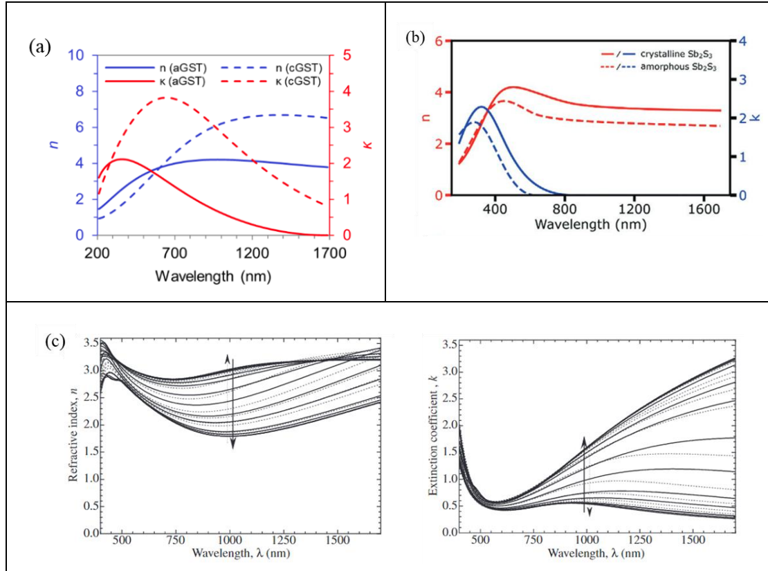
Figure 2.3. Optical properties of GST, VO 2 and Sb 2 S 3 in the Vis-NIR spectral range. (a) and (b) are the complex refractive index of GST and Sb 2 S 3 , respectively, as a function of wavelength in both amorphous and crystalline phases. [Zheng 2018; Delaney 2020] (c) Refractive index and extinction coefficient of VO 2 as a function of wavelength, respectively, at various temperatures between 25 and 120 °C. Solid and broken curves indicate the data obtained during the rise and drop in temperature, respectively. [Kakiuchida 2007]
