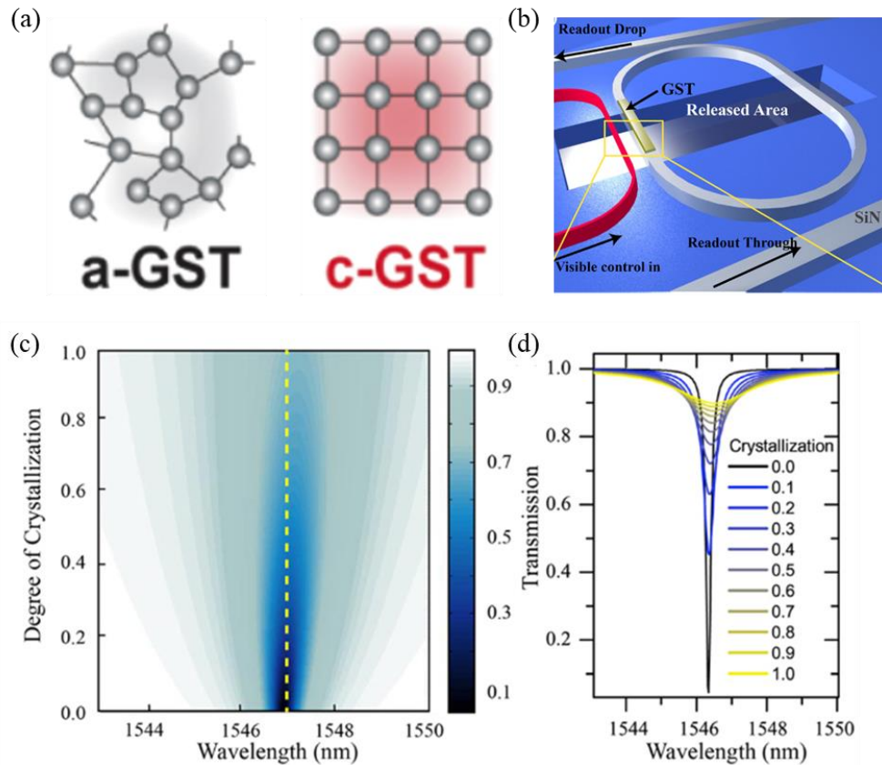
Figure 2.1. (a) Schematic structures of Ge 2 Sb 2 Te 5 (GST) in the amorphous (A) and crystalline (C) phases [Williams 2020] . (b) Schematic overview of the proposed GST-based integrated optical memory element. Light from a control port (red) is coupled evanescently to the ring resonator to perform the switching operation of the GST through photothermal heating. (c) The calculated transmission past the ring resonator as a function of the wavelength and the degree of crystallization of the GST. (d) The transmission at the cross-sectional line in (c), showing the increase in transmission as the ring shifts into the weakly coupled regime [Pernice 2012] .
