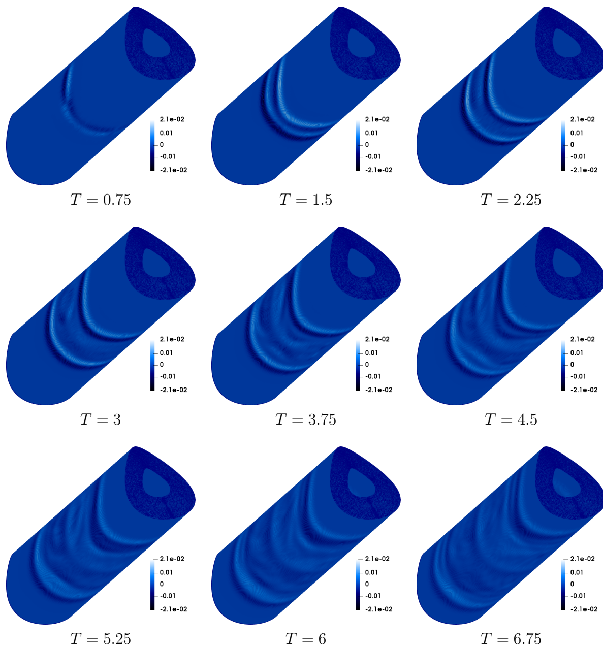
FIGURE 2.17 – The propagation of E_3 .
