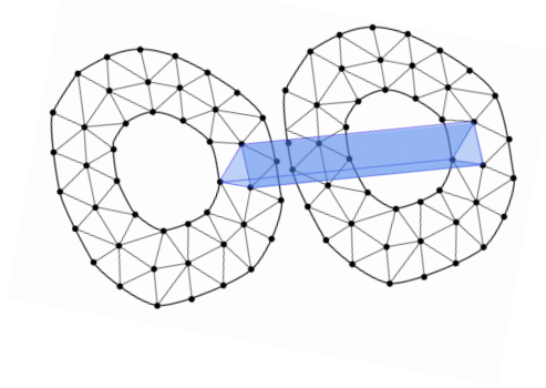
FIGURE 5.3 – Representation of a prismatic element in \mathcal{T}(\hat{\Omega}) (in blue a chunk of the infinite the prism \hat{P} ).
