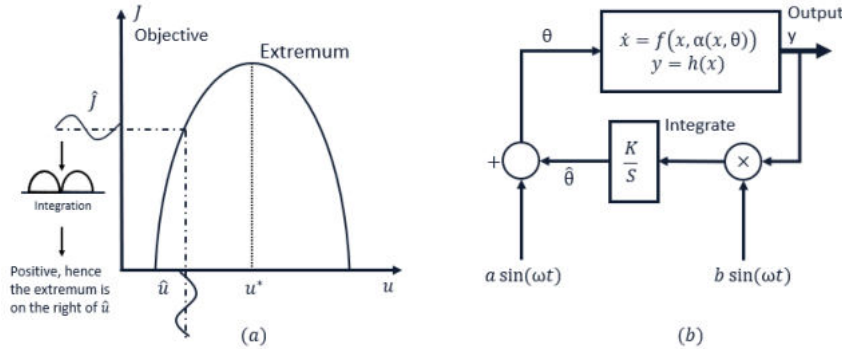
Figure 2.4: Illustration of the objective function J(\cdot) considered for this example (a) and the associated PB-ESC system (b).
