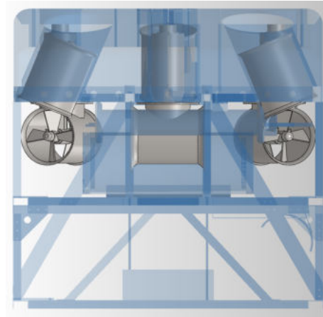
Figure 2.26: RexROV2 thruster positions, front view. Source: [Ber12].
