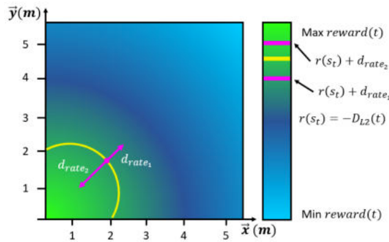
Figure 2.21: Spatial distribution of rewards in the (x, y) plane obtained with the reward defined in Eq. (2.89). The points that are at the same distance to the waypoint (i.e. yellow line) can now be associated with a different reward value based on the derivative of the distance.
