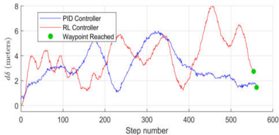
(b) Distance error d\delta from the ideal trajectory over time steps.
