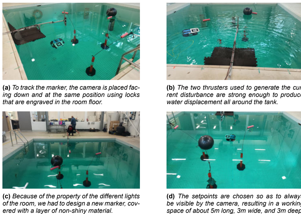
Figure 5.5: Illustration of the setup for the experiments.
