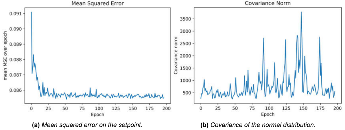
Figure 3.5: Training curves showing the evolution of the MSE and the covariance during training.
