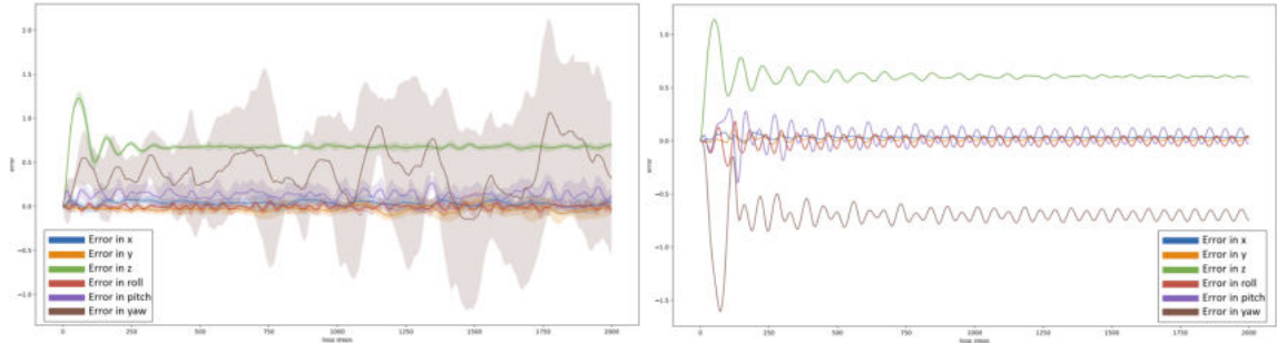
(c) The position and orientation errors of the LB PID during an episode from scenario 3. (d) The position and orientation errors of the naive PID during an episode from scenario 1.
