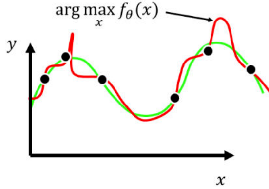
Figure 2.23: Imagine the green curve is the true function and the red curve is our fit. While the red curve is good in most cases, when we pick the maximum value of the function, we might pick out exactly that point where f(x) overestimates to a large degree (i.e. the largest positive error). This is similar to an adversarial example, in a particular direction.
