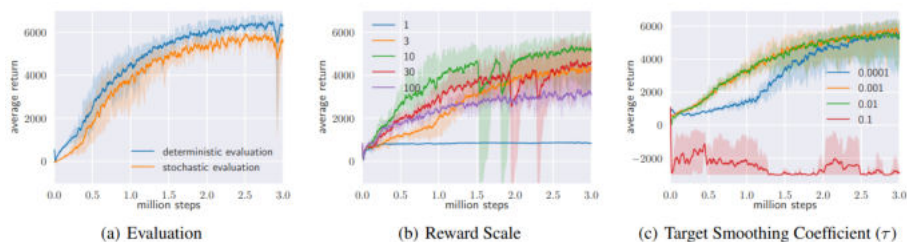
Figure 2.17: Illustration from [Haa+18c] of the sensitivity of the nominal SAC algorithm on the AntV1 task from the OpenAI gym benchmark suite [Bro+16].
