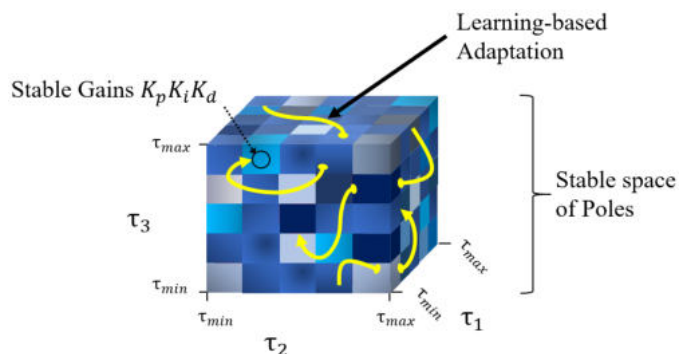
Fig. 1. Parameter cube representation for adaptive Pole-Placement control. The continuous space of possible poles is restricted to stable locations. It is explored by a deep reinforcement learning algorithm (yellow lines) that feed these parameters to a PID controller to derive the gains and thus the control law. This guarantees adaptability while converging to the steady-state.
