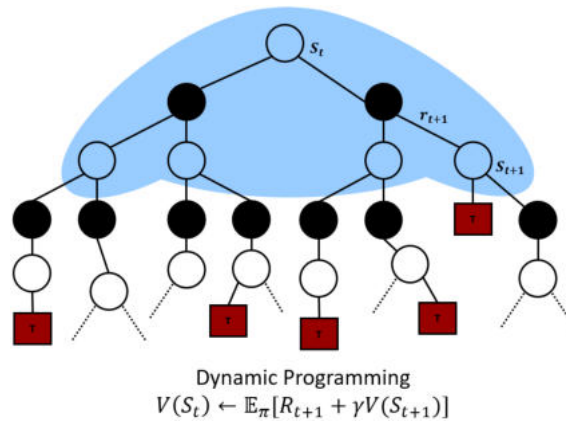
Figure 2.9: Backup diagram of DP-based method for the state-value function [SB18].
