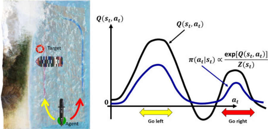
Figure 2.16: In maximum entropy reinforcement learning the policy is forced to explore the space of Q-Value more equally. This results in improved robustness to process variation as the agent is forced to explore sub-optimal strategies until the optimal long-term one is found.
