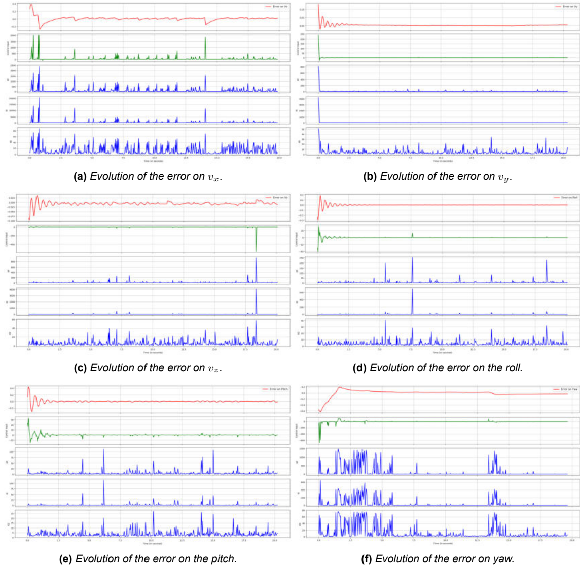
Figure 4.3: Evolution of the error on each DoF for an episode from scenario 5.
