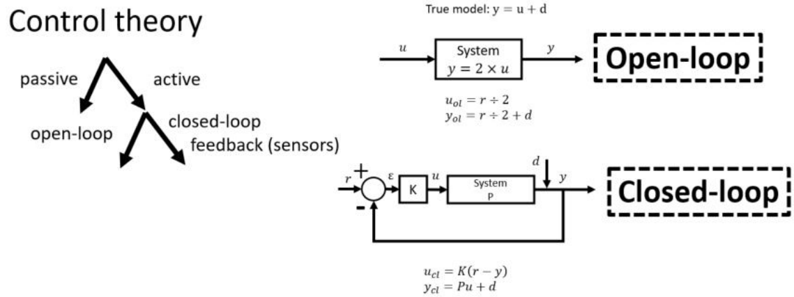
Figure 1.2: Control and dynamics are two sides of the same coin that are present in every aspect of our life. Control can be either passive or active, and allows us to ensure that our system of interest behaves as desired. The most common form of active control is known as closed-loop feedback control where the system output is measured and used to compute the next control input. As illustrated here, the closed-loop feedback controller is much more efficient at handling uncertainties and disturbances compared to its open-loop counterpart.
