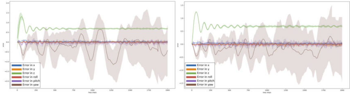
(a) The position and orientation errors of the LB PID during an episode from scenario 1. (b) The position and orientation errors of the LB PID during an episode from scenario 2.
