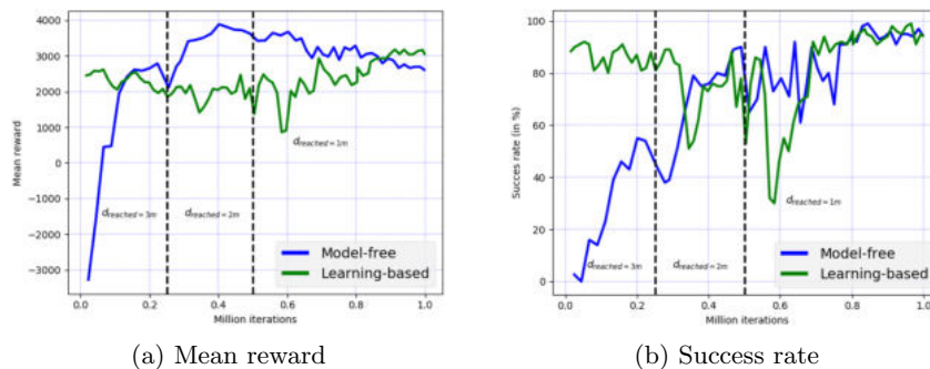
Fig. 5: Training curves showing the mean reward and success rate computed per 100 episodes over a moving window of 100 episodes. Note that with SAC, the policy is trained to maximize also the entropy, therefore the mean action does not always correspond to the optimal action for the maximum return objective.
