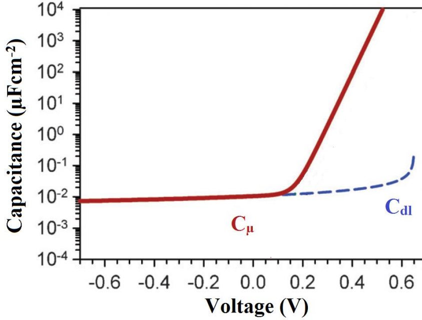
Figure IV. 24: Comparison between the chemical capacitance and the double layer capacitance
