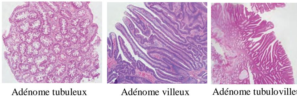
Figure 14 : Polypes adénomateux [33]
