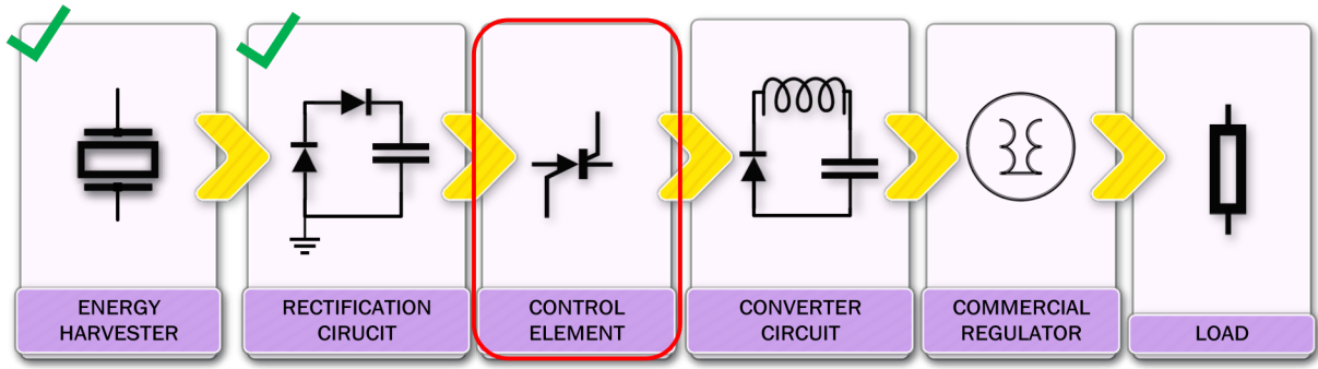
Figure 51: Proposed 5-stage system for energy harvesting and management adapted for use with commercial components. Progression to stage 3.
