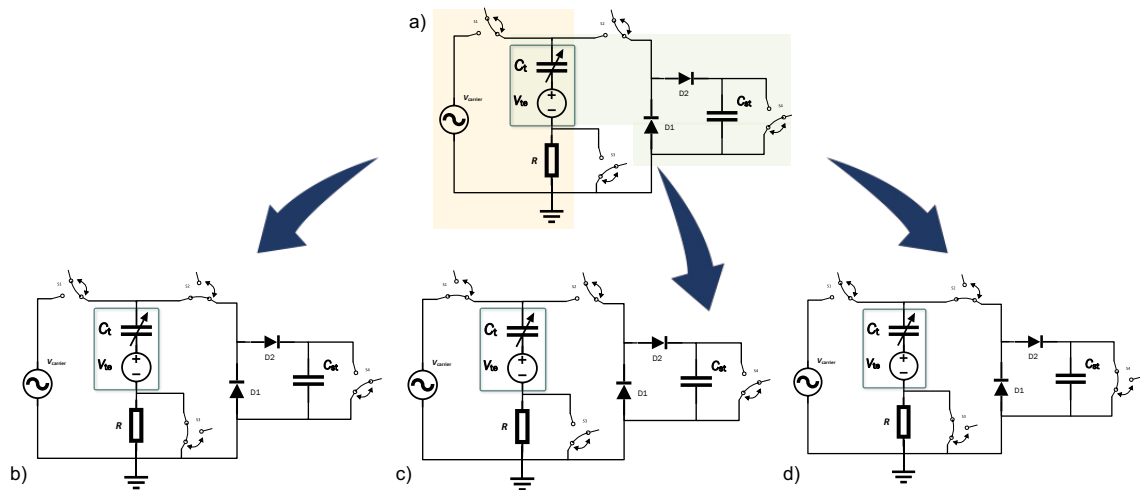
Figure 68: Schematic representation of components and their connection on the measurement board unit. a) The general schema of the board with all relays open. b) Case 2: S2 and S3 are closed, which corresponds to HW measurements. c) Case 1: S1 is closed forming a dynamic capacitance measurement circuit. d) Case 3: S2, S3 and S4 are closed. This schema discharges the output capacitor after an HW operation.
