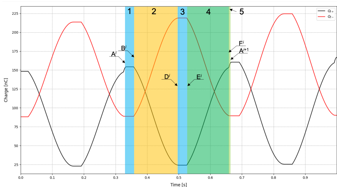
Figure 31: Simulation results for the charge levels of the C_{t+} and C_{t-} for the cycles 48-51.
