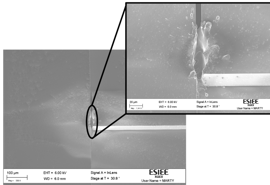
Figure 64: A closeup image of the level of damage created on the tested switch. Destruction of materials contracting anode and cathode and fusion of the two.
