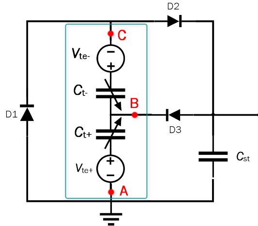
Figure 18: Schematic of "double TENG" - "double Bennet" circuit system.
