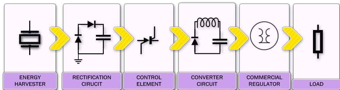
Figure 1: Proposed 6-stage system for energy harvesting and management adapted for use with commercial components.
