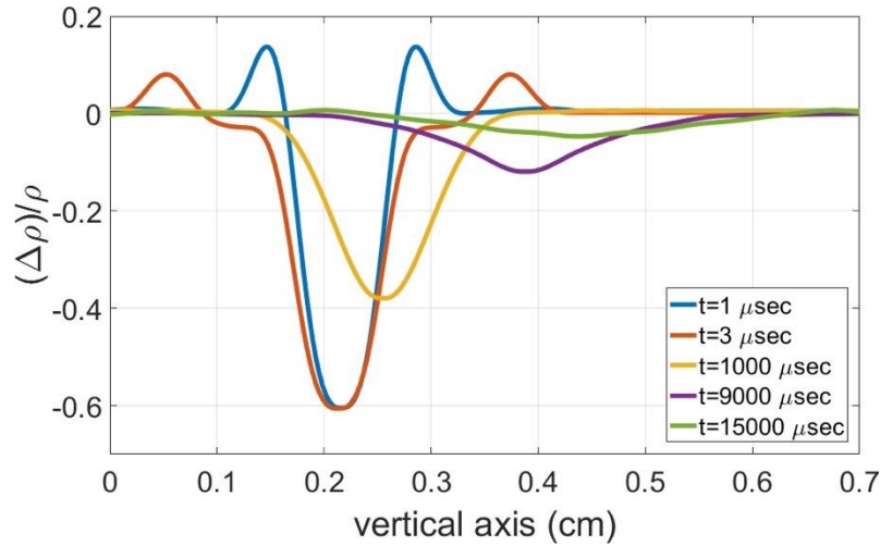
Figure 2.2.1: Profile of the density variation of the under-dense channel measured at different delays after its creation, ranging from 1 \mu\text{s} to 15 ms.
