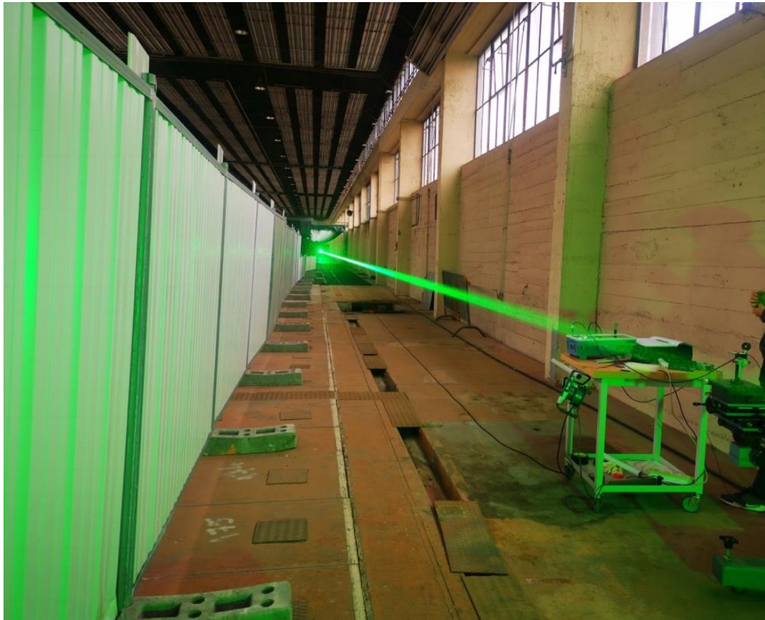
Figure 1: Picture of the frequency doubled beam propagating along the 140 m experimental zone.
