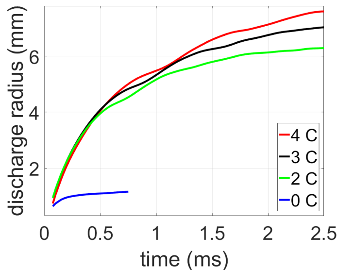
Figure 2.3.5: Measured temporal evolution of the discharge radius for capacitance values in the secondary circuit of C = 720 nF (labelled as 4C, in red), C = 540 nF (labelled as 3C, in black), C = 350 nF (labelled as 2C, in green), and for no capacitance (labelled as 0C, in blue).
