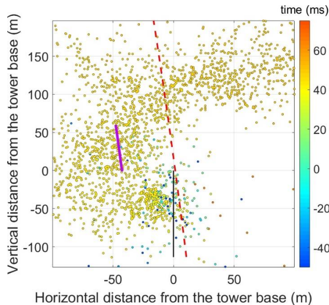
Figure 4.7.2.1: 2D maps of the VHF sources emitted during the lightning event N06. The Säntis tower is represented on each plot as a black line, the laser path is represented as a red dotted line. Each point corresponds to a VHF emission. The delay between the VHF source and the initiation of the current on the tower is shown by the color code displayed on the right. The violet line shows the region where the channel resulting from the laser filamentation would be located after the wind moved it during 3 s.
