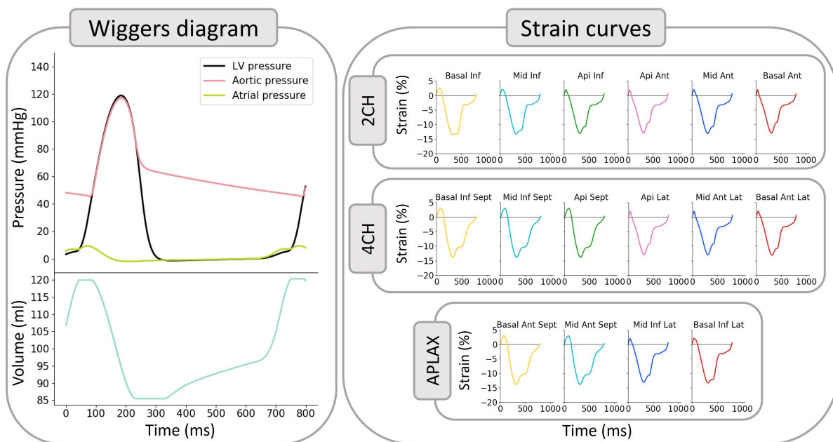
Figure 3.8: Model simulation example results in healthy conditions adapted from [41]. Wigger diagram : left ventricle (black), aortic (pink) and atrial pressure (green) and LV volume (blue). On the right, the Strain curves : 16 LV segments strain signals for the 3 views (2CH, 4CH and APLAX).
