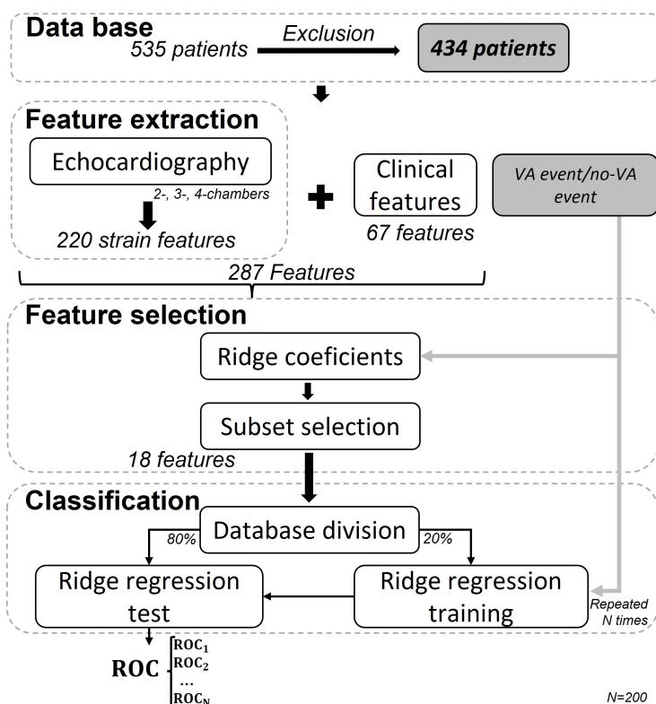
Figure 6.3: Machine learning pipeline. Clinical information and data extracted from LV longitudinal strain curves were collected for 434 HCM patients. Among the 287 features extracted (220 strain-derived), a sub-selection of the most discriminating features was made according to ridge coefficient order. Finally, the final performance of the model is obtained after a repeated cross validation step.
