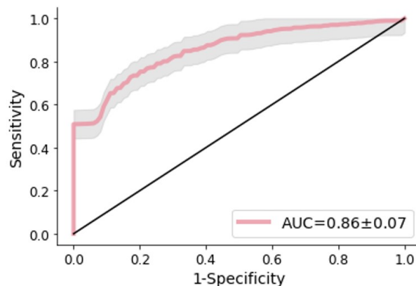
Figure 4.20: ROC curve of the RF classifier on model-extracted features with the 22 first features, 500 estimators and 200 cross-validation repeats. The AUC is computed on the 200 test datasets.
