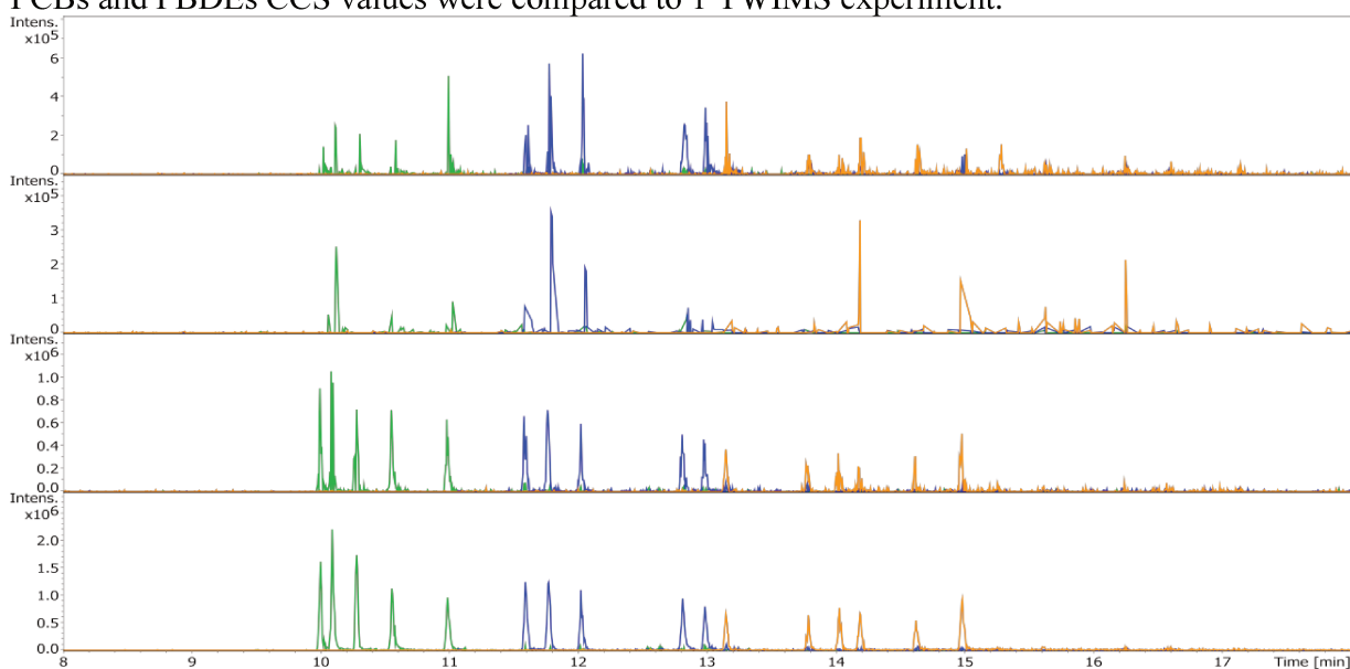
Figure 8 Protonation of PBDE- Br 4-6 . It indicated an unstable and irreproducible of protonation ion under APCI source. The relative response ratios within isomers were not consistent. Not all the protonation ions can be observed by repeated injection.
