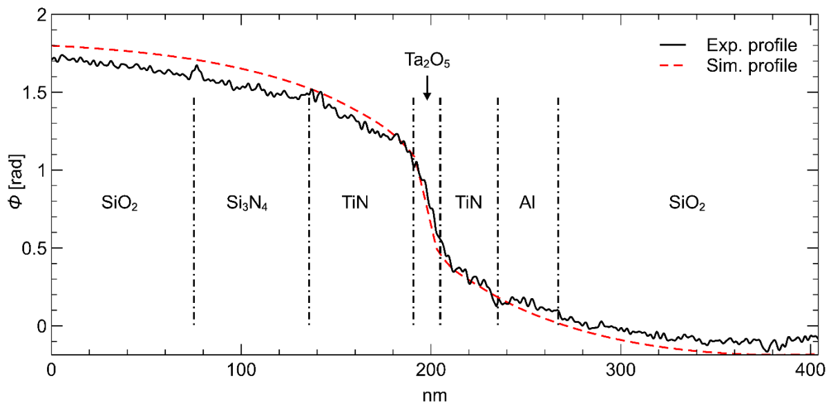
Figure 6.4 : Extracted profiles of experimental and simulated phase images along the black arrows on the phase images Figure 6.3b, c.
