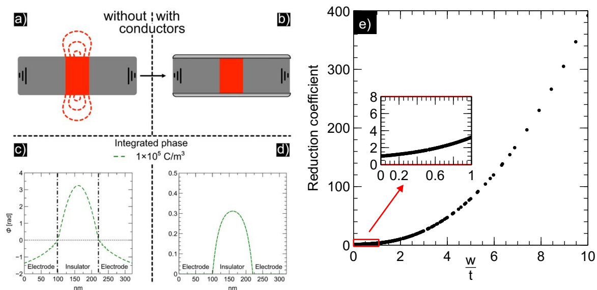
Figure 3.21 : Effect of the conductive layers in surface to a model capacitor. Left: schemes a), b) and phase profiles for each case respectively c), d). Right, the reduction coefficient as a function of the aspect ratio e).
