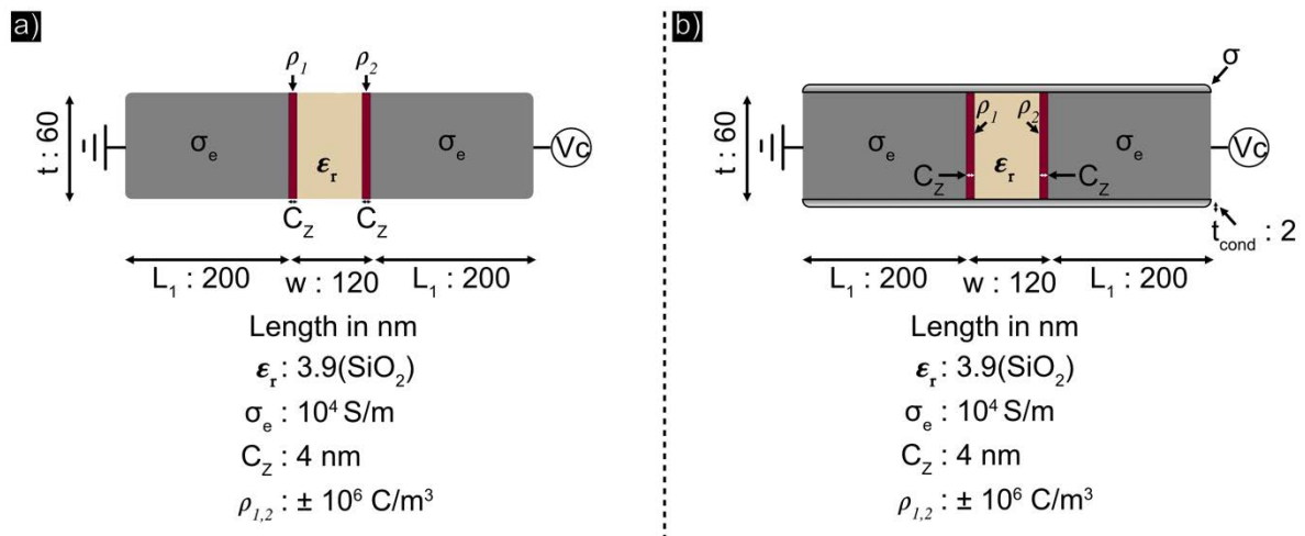
Figure 3.32 : Biased capacitors with charged density into the dielectric at these electrode interfaces without a) and with conductor layers b).
