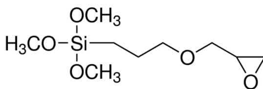
Figure 5.5: 3-Glycidyloxypropyl trimethoxysilane.
