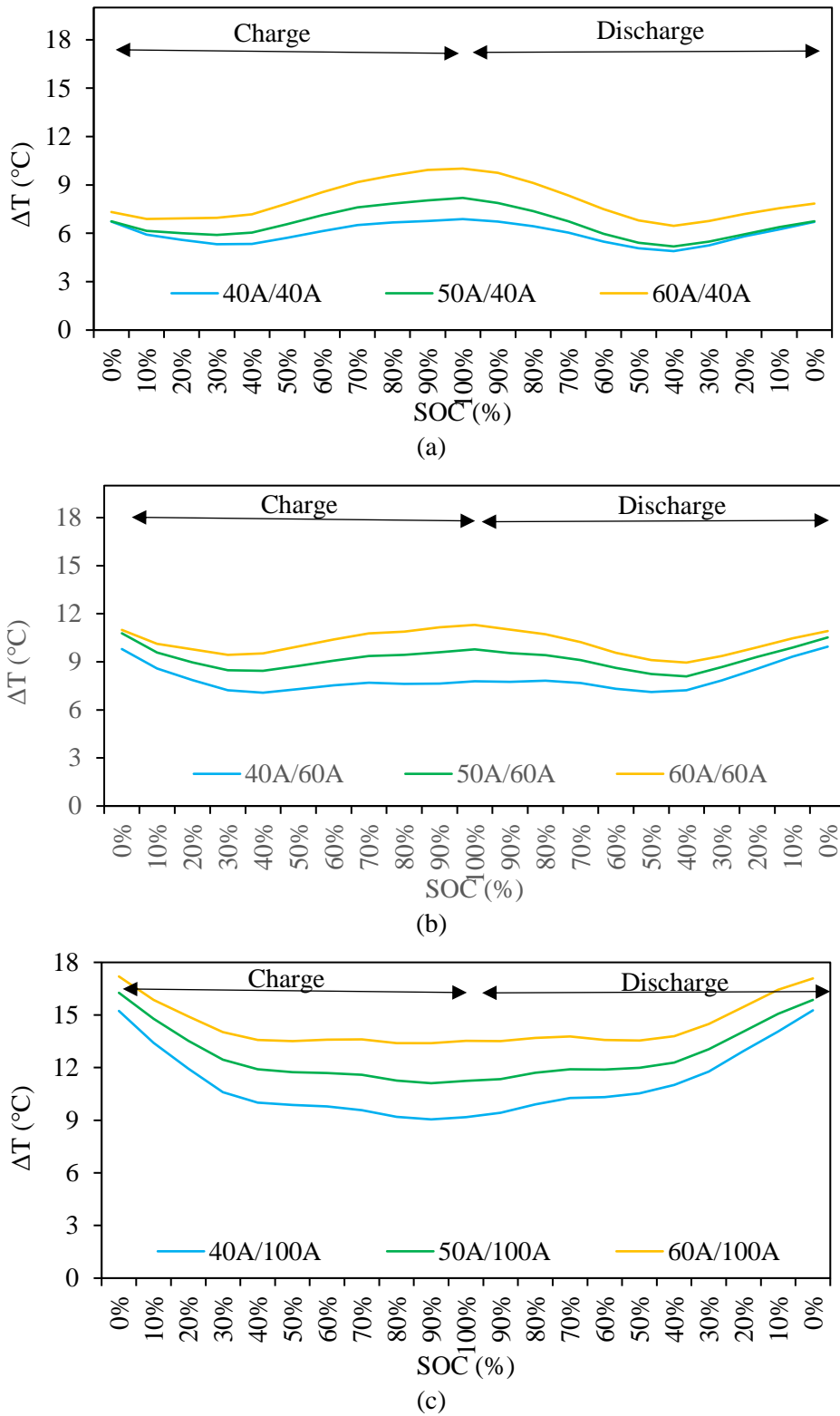
Figure II.22 Temperature profiles during quasi stationary regime versus SOC: (a) I_d=40 A, (b) I_d=60 A, (c) I_d=100 A.
