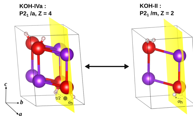
Figure 3.3: Sketch of the symmetry changing for \text{KOH-IVa} \leftrightarrow \text{KOH-II} phase transition using crystallographic data from reference [113].
