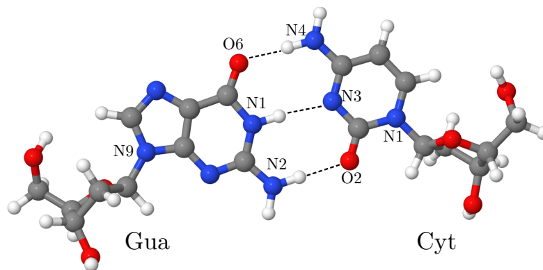
Figure 5.3: Representation of the canonical Watson-Crick deoxyguanosine and deoxycytosine nucleoside pair (dG-dC) employed in the current AMOEBA18 calculations. The oxygen, nitrogen, carbon and hydrogen atoms are colored red, blue, grey and white respectively.
