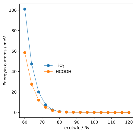
Figure C.1: Convergence respect to the energy cutoff for the wavefunctions.
