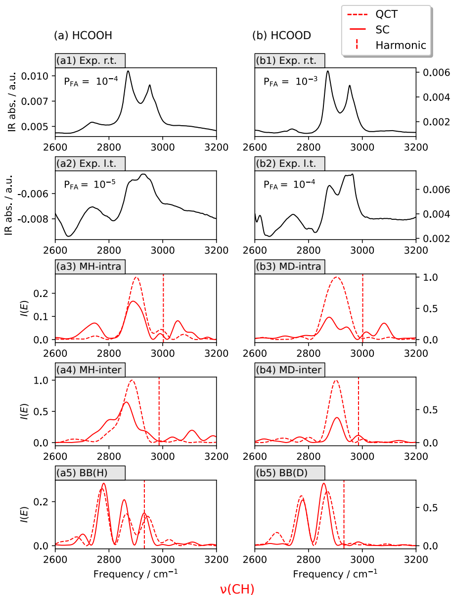
Figure 4.12: The QCT and SC power spectra of CH stretching vibration of adsorbed FA compared with the low- (LT) and room-temperature (RT) FT-IR spectra at a selected partial pressure P_{\text{FA}} (mbar). Left: HCOOH adsorption; right: HCOOD.
