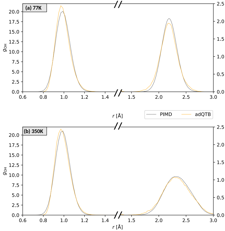
Figure 3.15: Radial distribution function for OH pairs from PIMD and adQTB simulations. Panel (a): low-T. Panel (b): high-T.
