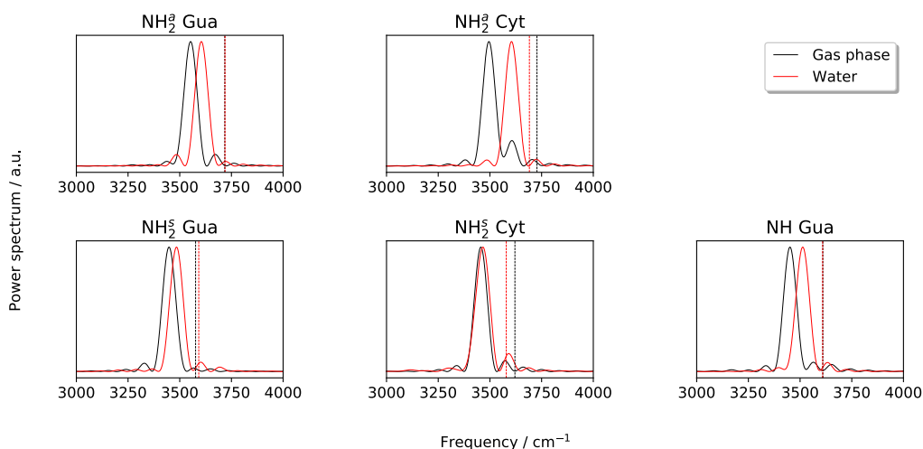
Figure 5.7: QCT spectra of interbase NH stretching vibrations in gas phase and solvated dG·dC using AMOEBA/BIO18. The corresponding harmonic values are reported as vertical dashed lines.
