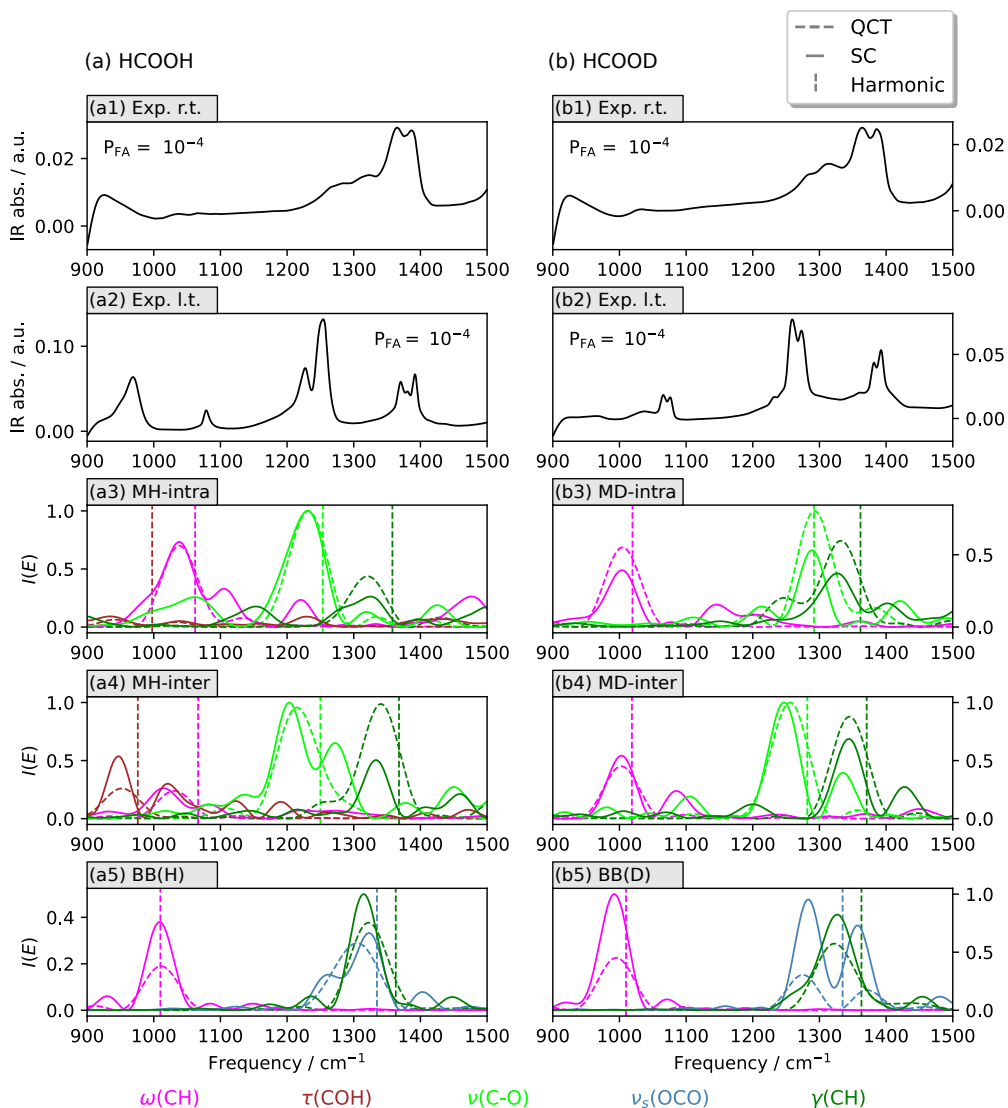
Figure 4.10: The QCT and SC power spectra of the fingerprint region of adsorbed FA compared with the room- (r.t.) and low-temperature (l.t.) FT-IR spectra at a selected partial pressure P_{FA} (mbar). Left: HCOOH adsorption; right: HCOOD.
