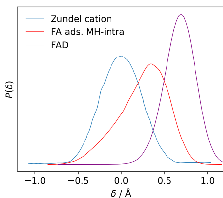
Figure 4.20: Probability distribution at T = 100 K of proton sharing coordinate \delta in (I) zundel cation from Shran et al. [191] (Figure 4, curve at 2.4 \text{ \AA} ), (II) formic acid adsorbed on anatase (101) surface in monodentate mode (intra) and (III) formic acid dimer using PES from Qu et al. [190].
