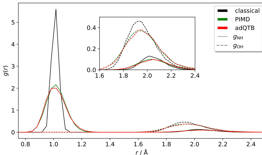
Figure 5.4: Radial distribution function g(r) of NH and OH interbase pairs of gas-phase dG-dC at 300 K from adQTB, PIMD and classical Langevin simulations using AMOEBA18.
