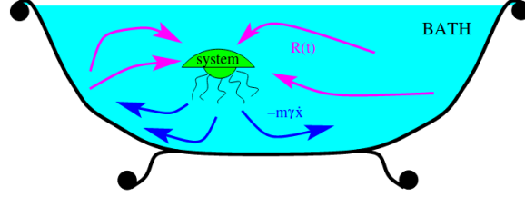
Figure 2.9: The Langevin equations eq. (2.71) as a thermal bath in classical molecular dynamics simulations. Reproduction from reference [91].
