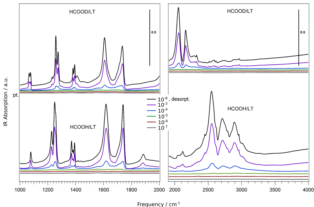
Figure 4.8: FTIR spectra at low temperature (13 K) of protonated FA vs deuterated FA adsorbed on anatase \text{TiO}_2 nanopowders exposed to P_{\text{FA}} = 10^{-7}\text{-}10^{-3} mbar, compared to the spectra recorded after FA desorption at P_{\text{FA}} = 10^{-8} mbar (black curve).
