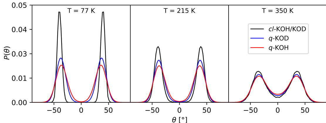
Figure 3.9: Probability distribution for the microscopic order parameter \theta from ab initio classical ( cl -KOH/D) and PIMD simulations ( q -KOH and q -KOD). The distributions have been symmetrized.
