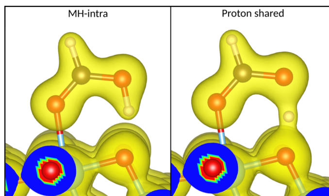
Figure 4.5: Charge electron density associated to the MH-intra mode (left) and the proton shared configuration (right). The isodensity used to generate this figure is equal to 0.1 e/\text{\AA}^3 .
