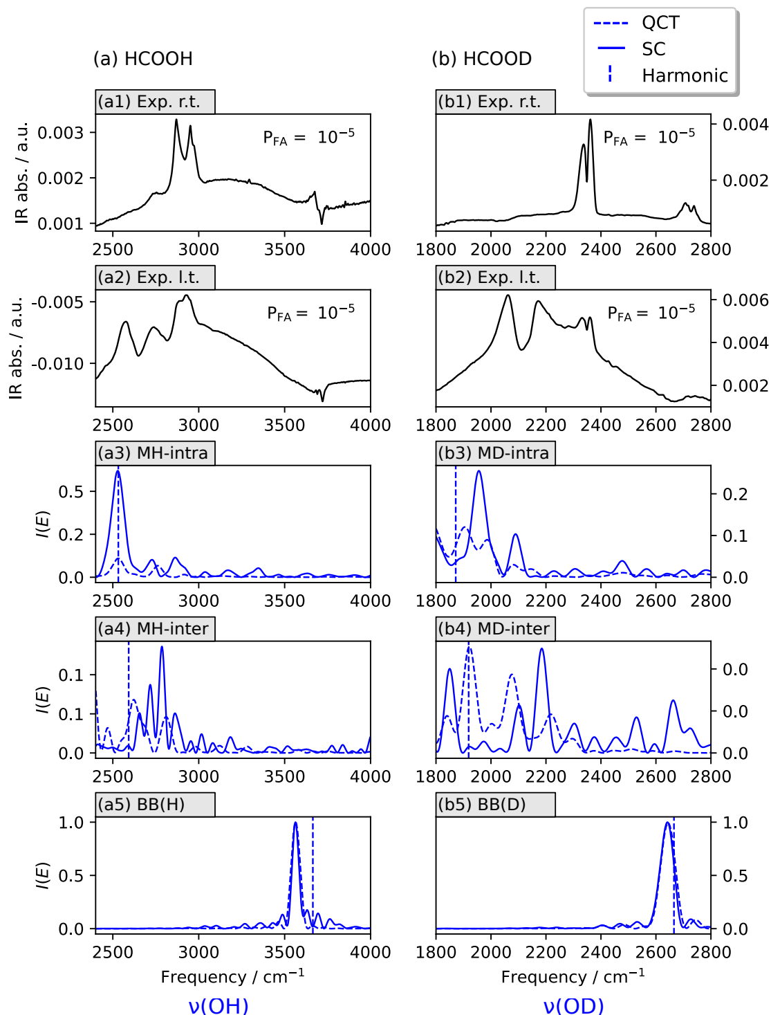
Figure 4.14: The QCT and SC power spectra of OH and OD stretching vibration of adsorbed FA compared with the room- (r.t.) and low-temperature (l.t.) FTIR spectra at a selected partial pressure P_{\text{FA}} (mbar). We remind that the doublet at \sim 2300 \text{ cm}^{-1} is due to the \text{CO}_2 present in the chamber. Left: HCOOH adsorption; right: HCOOD. All the QCT and SC refer to a single classical trajectory with \alpha = 1 , except MH-intra ( \alpha = 3/4 ) and BB(D) ( \alpha = 1/2 ).
