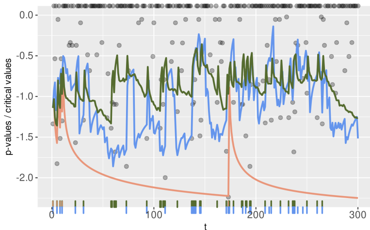
Figure 2.4: Sequences of critical values of LORD procedure with different rewards over time 1 \leq t \leq T = 300 (simulated data): base LORD critical values (B.13) (orange line), rewarded with the greedy approach (2.24) (blue line), and with the rectangular kernel SUR spending sequence (2.25) ( h = 10 , green line). The rug plots display the time of discoveries for each procedure with the corresponding color. The y -axis has been transformed by y \mapsto -\log(-\log(y)) . The grey dots denote the p -value sequence (those equal to 1 are displayed at the top of the picture). The spending sequence is \gamma_t \propto t^{-1.6} .
