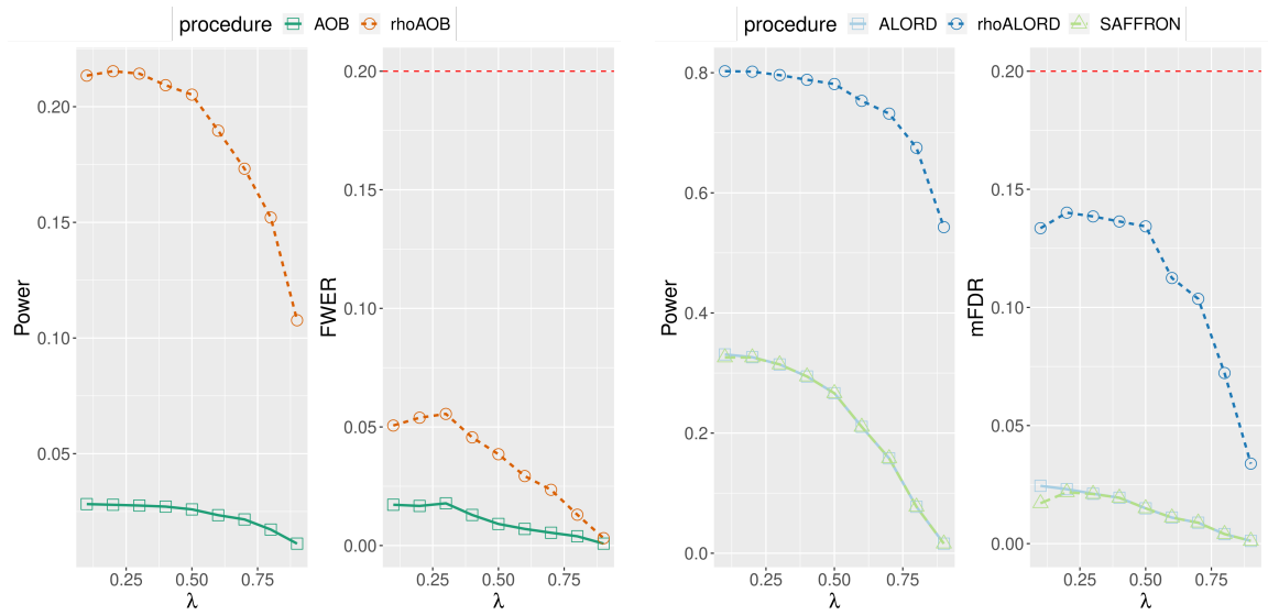
Figure A.7: Power and type I error rates, for the considered procedures, versus the adaptivity parameter \lambda .
