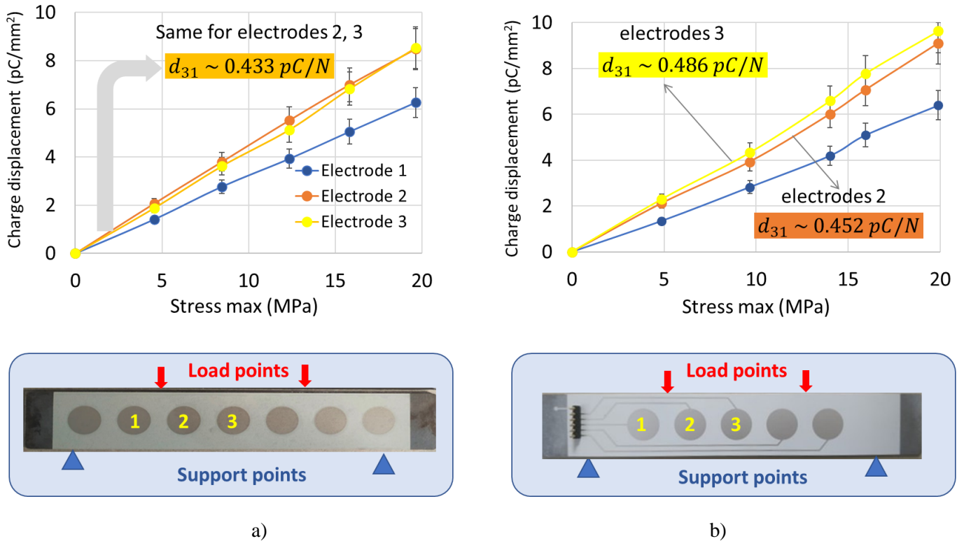
Figure 3.9. Charge displacement versus stress of sample: a) without printed conductive tracks; and b) with printed conductive tracks.
