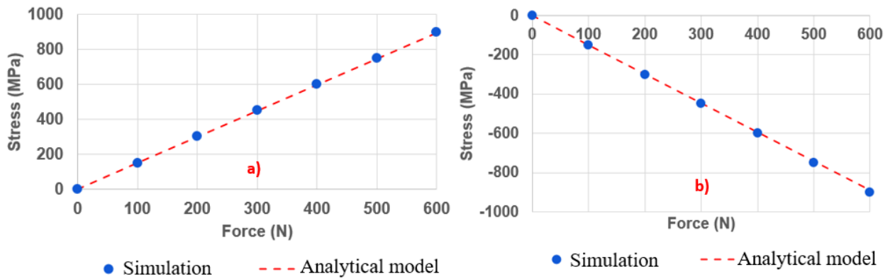
Figure 3.4: Comparison of mechanical properties between analytical model and simulation: a) b = 120\text{ mm} , L = 150\text{ mm} ; b) b = 150\text{ mm} , L = 120\text{ mm} . Dashed lines represent the analytical model according to Eq. (2.3), while dotted symbols display the simulation data.
