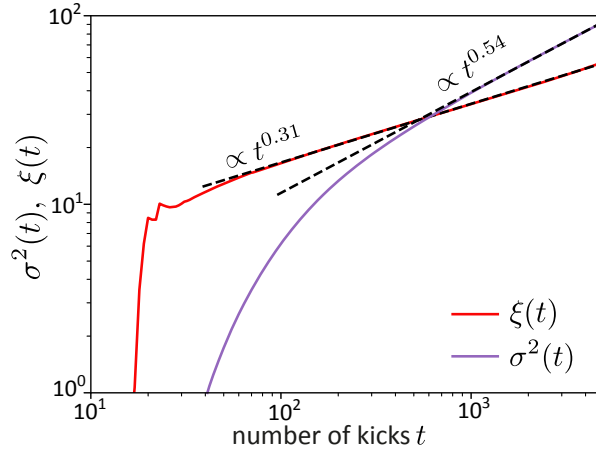
Figure 5.6: Time evolution of the exponential decay length \xi(t) governing the far tails of the momentum distribution. A linear fit (dashed line) suggests an algebraic scaling close to \xi(t) \sim t^{1/3} . The time evolution of the mean square width \sigma^2(t) is also shown for comparison. Here f = 16 , \gamma^* = 4 and \lambda = 3.03 .
