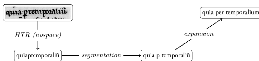
Fig. 2. Workflow for the full modular approach [6]. The digital image is segmented in lines that are submitted to recognition, and the recognised text then goes through word segmentation and normalisation (abbreviation expansion).
