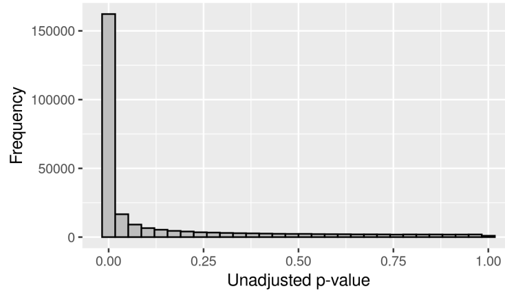
Figure 4.10: Histogram of unadjusted p -values
