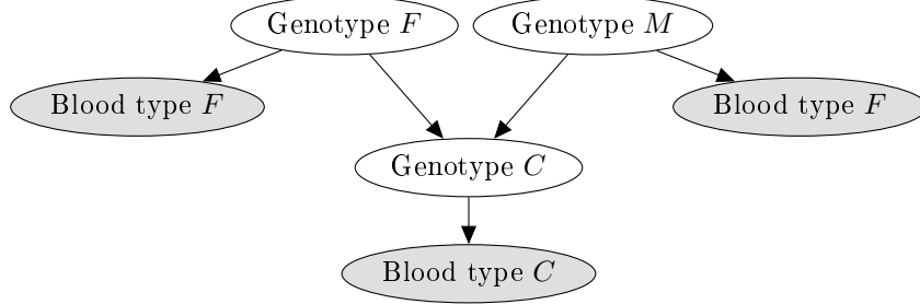
Figure 2.2: Directed acyclic graph
