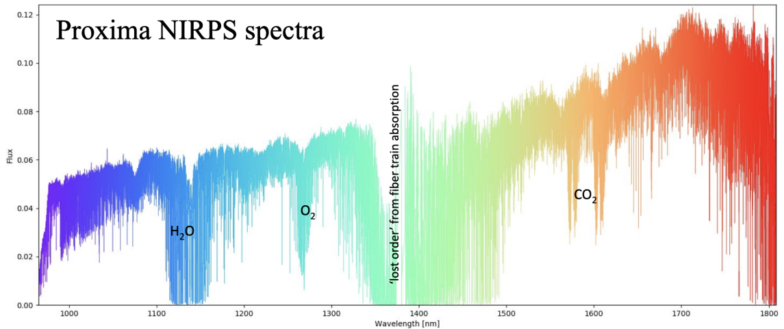
Figure IV.16: Spectrum of Proxima from the NIRPS spectrograph.
