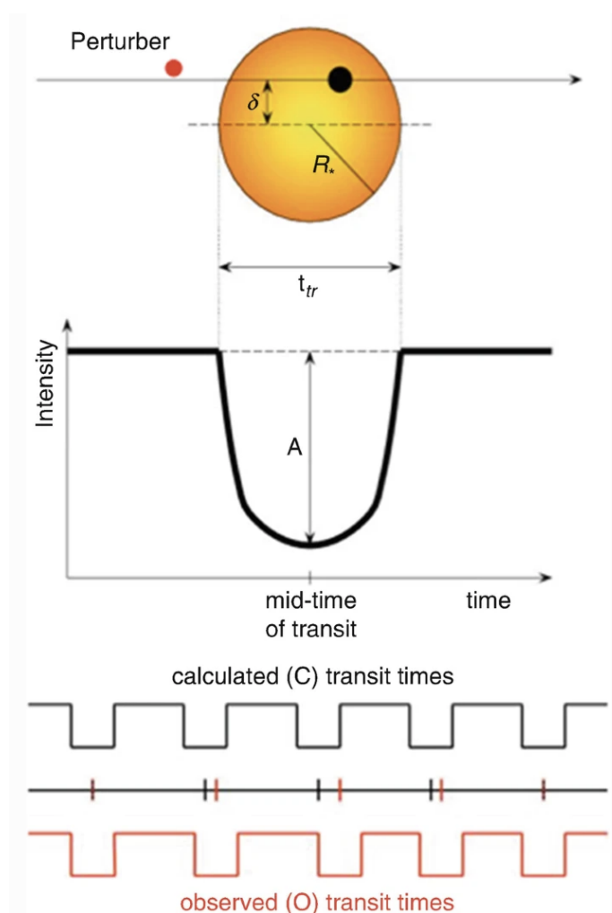
Figure III.16: TTVs.
