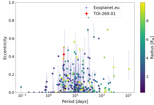
Fig. 15. Orbital eccentricity as a function of the orbital period with the planetary radius (see color scale at right) from the Exoplanet.eu catalog.
