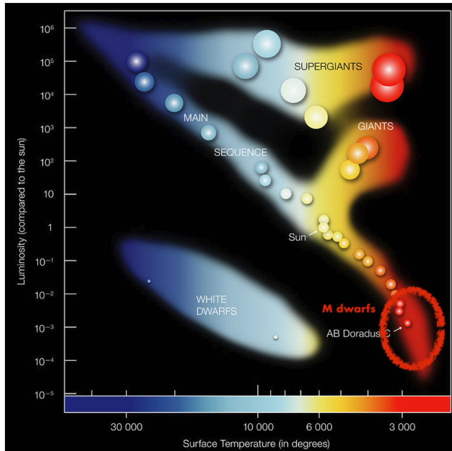
Figure I.7: Hertzsprung-Russell diagram.
