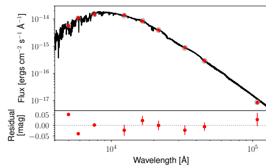
Fig. C.1. Spectral energy distribution of TOI-269. The solid line is the MAP PHOENIX/BT-Settl interpolated synthetic spectrum, red circles are the absolute photometric observations, and gray open circles are the result of integrating the synthetic spectrum in the observed band-passes.
