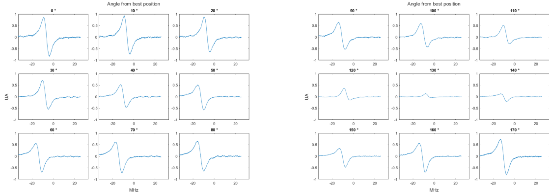
Figure 3.5: MTS signal after demodulation as the polarisation of the probe going into the fiber is changed. The polarisation is changed by turning a half-waveplate, the angle represented on top of the figures is the angle of the half waveplate from the optimized error signal position. The error signal is scanned by sweeping the laser's frequency and recorded. This measurement is repeated as the polarisation of the probe injected in the fibre is changed. The MTS signal is demodulated with a 5 kHz bandwidth.
