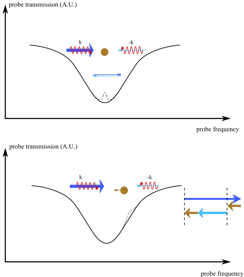
Figure 1.7: Representation of the SAS velocity class selection. The Doppler broadened profile can be reduced by addressing only one class of speeds in the cloud. In order to do so, a beam is send in one direction, saturating one class of speed. When another beam is sent through the medium, the transmission profile will show a local maximum for this saturated velocity class. (a) When both pump and probe have the same frequency, the Lamb dip is centered on the zero velocity class (b) for different frequencies of pump and probe a certain non zero velocity class can be resonant simultaneously with both beams. Most of the time, retroreflected beams are used to address the zero velocity class.
