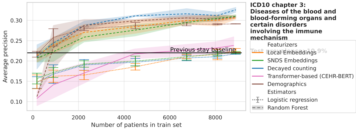
Fig. C.20. ICD10 chapter 3
