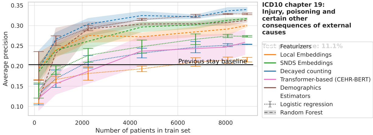
Fig. C.19. ICD10 chapter 19
