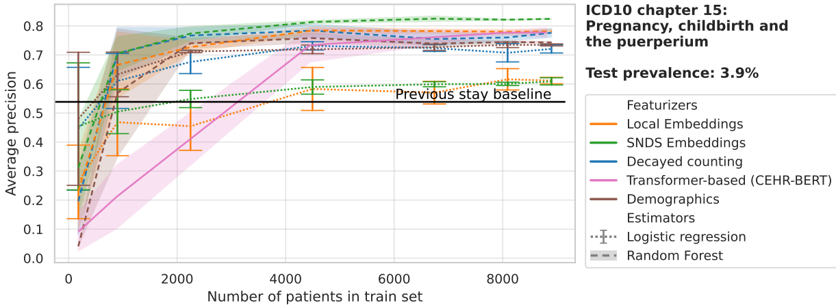
Fig. C.26. ICD10 chapter 15
