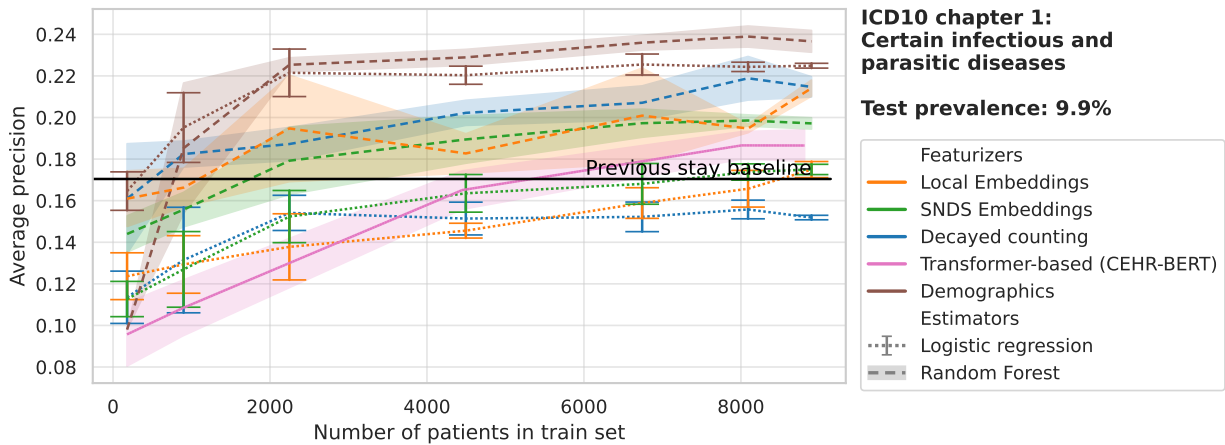
Fig. C.21. ICD10 chapter 1
