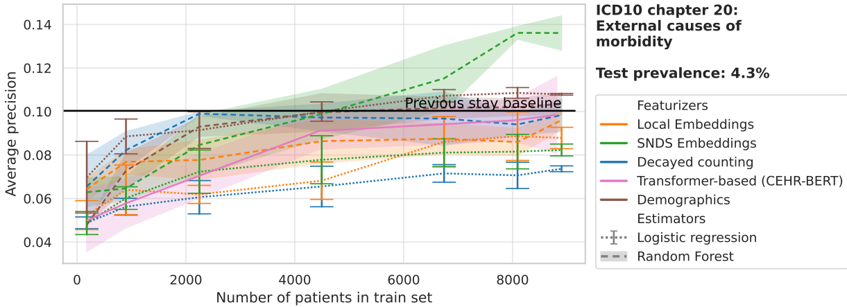
Fig. C.25. ICD10 chapter 20
