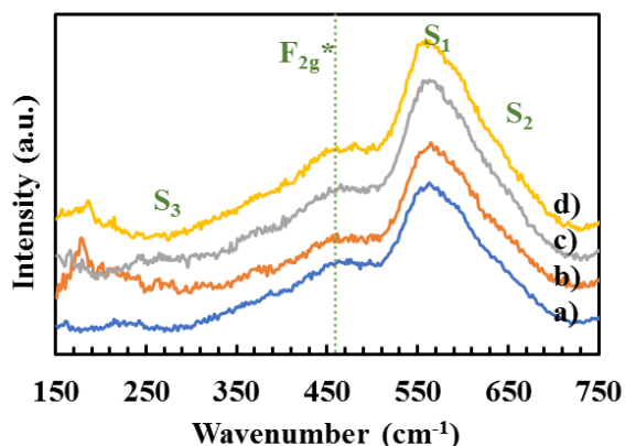
Figure 77 Raman spectra for \text{CeNi}_x\text{Zr}_{0.5}\text{O}_y calcined catalysts after 31 hours test with a pretreatment in \text{H}_2 at 200\text{ }^\circ\text{C} : a) x = 0.5 , b) x = 1 , c) x = 2 and d) x = 5 .
