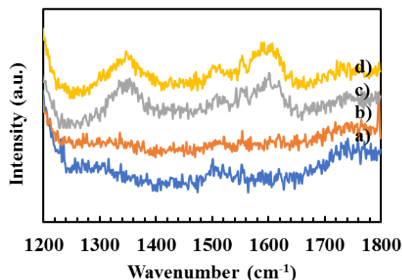
Figure 78 Raman spectra in the carbon region for \text{CeNi}_x\text{Zr}_{0.5}\text{O}_y calcined catalysts after 31 hours test with a pretreatment in \text{H}_2 at 200\text{ }^\circ\text{C} : a) x = 0.5 , b) x = 1 , c) x = 2 and d) x = 5 .
