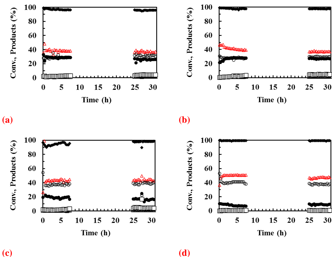
Figure 24 Ethanol conversion (♦) and products distribution (H 2 △, CO 2 ○, CO ●, CH 4 △, acetaldehyde □) after 31 hours in OSRE on CeNi x Zr 0.5 O y dried catalyst in-situ pretreated in H 2 at 200 °C. a) x = 0.5, b) x = 1, c) x = 2 and d) x = 5. Conversion of O 2 not reported is total (EtOH/H 2 O/O 2 /N 2 = 1:3:1.7:N 2 ).
