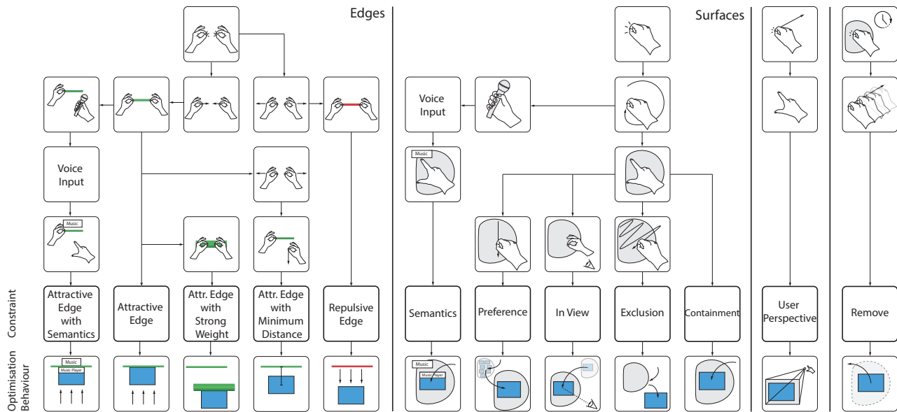
Figure 4.8: Complete diagram describing the final set of gestures of our system. All gestures begin from one of the four states shown at the top, each following a unique path to the constraints at the bottom.
