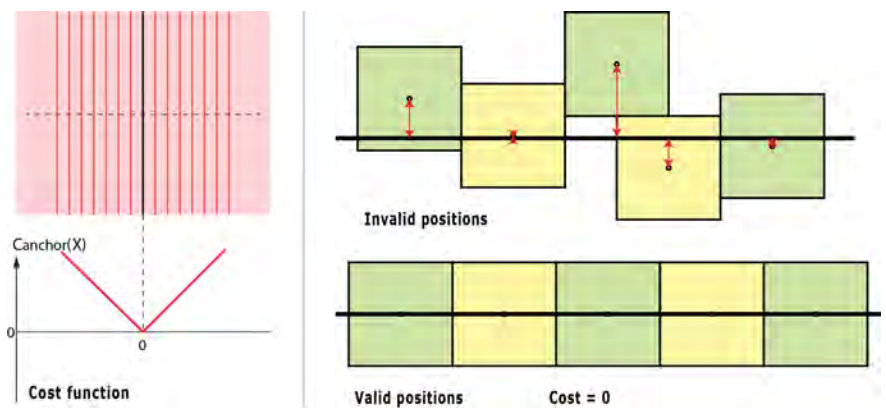
Figure 3.7: Cost function of an alignment constraint and value of the cost according to decal position
