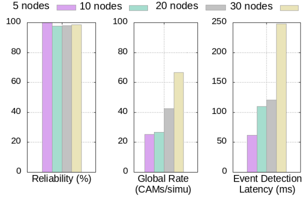
Figure 5.8: ETSI Standard Performance.
