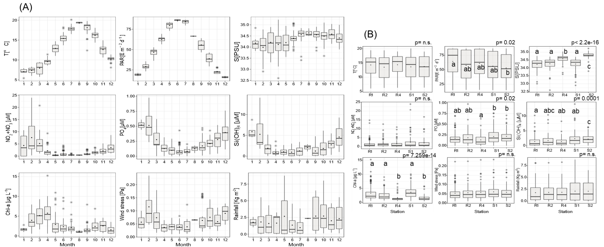
Figure S2.2. (A) Monthly variations of the environmental variables: Temperature ( T , °C), Photosynthetic Active Radiation (PAR, E m^{-2} d^{-1} ), Salinity ( S , PSU), nitrite and nitrate ( NO_2+NO_3 \mu M ), phosphate ( PO_4 , \mu M ), silicate ( Si(OH)_4 , \mu M ), chlorophyll-a ( Chl-a , \mu g L^{-1} ), wind stress ( Pa ), rainfall ( Kg m^{-2} ) (B) Spatial variations of the environmental variables measured in the eastern English Channel at the DYPHYRAD and SOMLIT stations from March 2016 to October 2020. The letters indicate significant differences ( p < 0.05 ) between stations based on Kruskal-Wallis and Nemenyi post-hoc test on the top of the graphs. Solid black lines represent the median, black dots the mean and the black stars the outliers.
