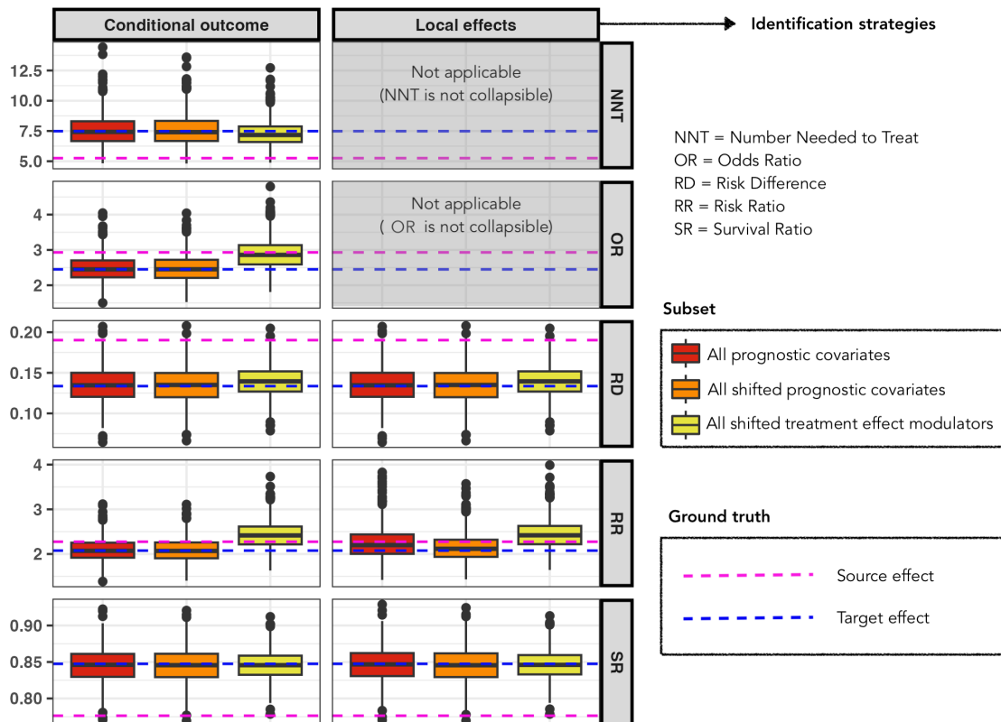
Figure 5.6: Simulation with binary outcome Y : for a monotonous and deleterious effect. Therefore conditions of Lemma 15 are satisfied, allowing to generalize the Survival Ratio with fewer covariates, and in particular only shifted treatment effect modulators , here stress. Adding all shifted prognostic covariates (stress and lifestyle), or even more with all prognostic covariates (stress, lifestyle, and gender) enables generalization of all causal measures by generalization of the conditional outcome or re-weighting of local effect if possible (only for collapsible measures, namely RR, SR, and RD). On this simulation, estimation is done with IPSW estimator, source (resp. target) sample being of size n = 5\,000 (resp. m = 20\,000 ), with 1 000 repetitions.
