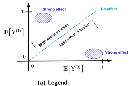
Figure 5.7: Plots a of the ranges of the different metrics as a function of the proportion of events in control group, namely \mathbb{E}[Y^{(0)}] (x-axis), and of the proportion of events in treated group, namely \mathbb{E}[Y^{(1)}] (y-axis). See Subfigure 5.8a. As both the colors and the different scale illustrate, the ranges of the effect considerably differ with the metric chosen. Note that for the NNT (Figure 5.7b) we only represented the quarter of the plot when an event encodes death.
