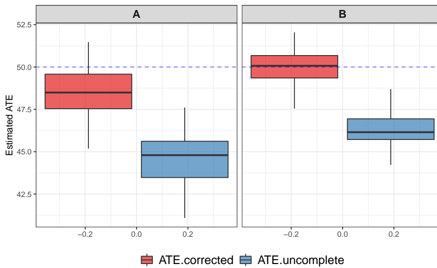
(c) ATE estimation in the two situations where \hat{\tau}_{G,obs} is estimated considering X_1 is missing and denoted ATE.uncomplete, while the bias B is estimated following Theorem 5 giving ATE.corrected ( \hat{\tau}_{G,obs} + \hat{B} ).
