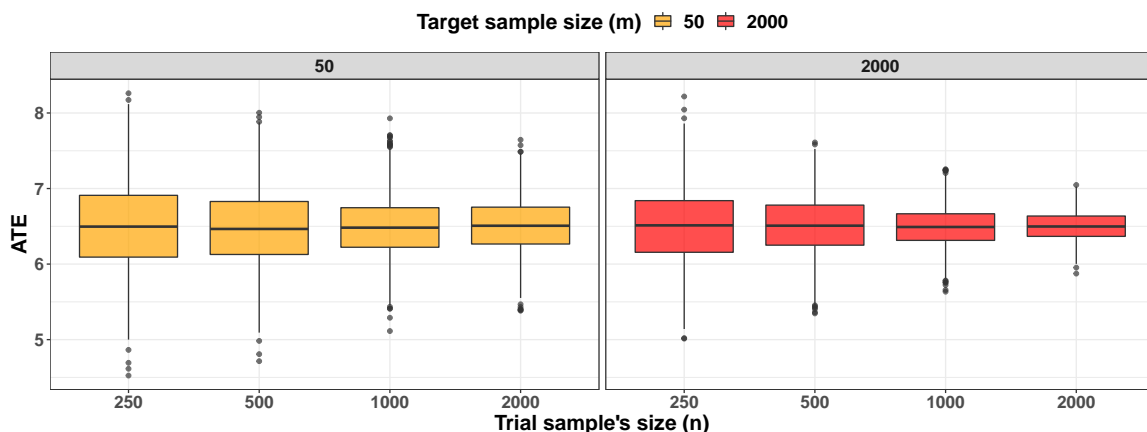
(c) Two data sets leading to two asymptotic regimes: where two situations are considered, one with a large target sample ( m = 2000 ) or a small target sample ( m = 50 ). Then, increasing n leads to a variance stagnation if m is small, while increasing n allows to further gain in precision if n \leq m .
